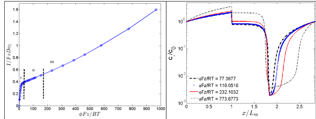
Figure 7.6: (a) Normalized current–voltage characteristics (in magnitude) of a cation–selective nanochannel connected to two microchannels. (b) Normalized concentration of anions (co–ions) along the axial direction for various DC voltages, corresponding to the limiting resistance and overlimiting region.
