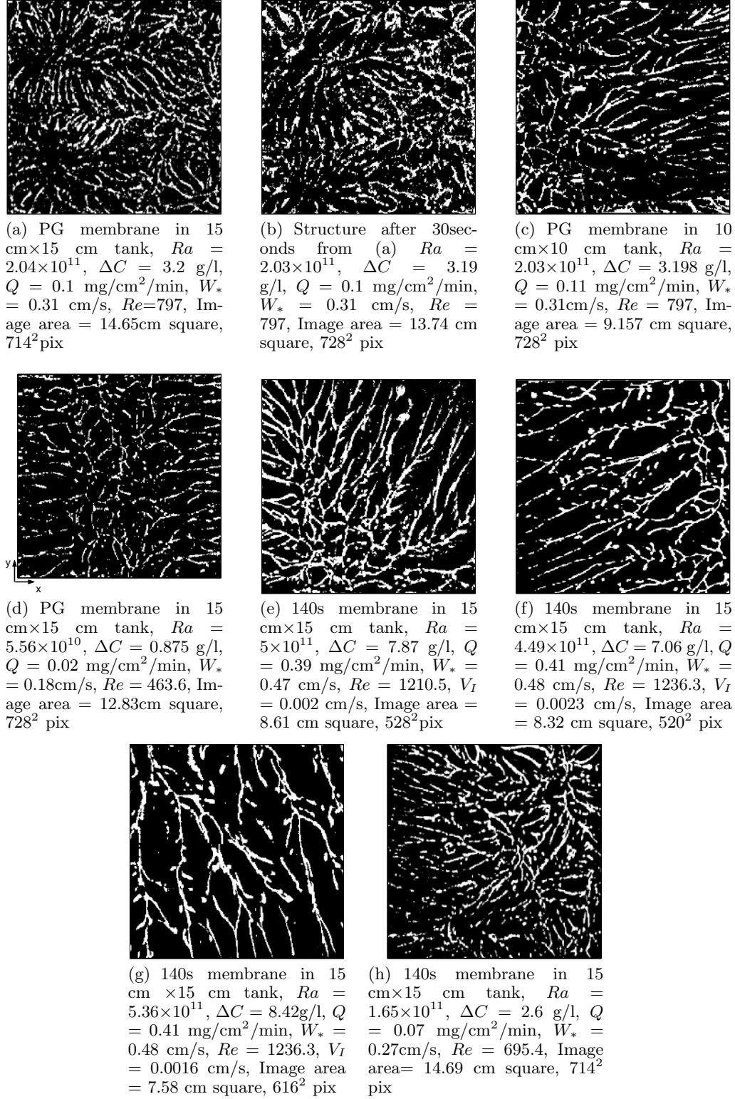
FIGURE 2. The plan forms of near wall plume structures obtained under different conditions. (a) to (d) are for the D-Type showing full tank cross section. (e) to (g) show the planforms of the plume occupied region in the TF-type convection. (e) shows the corner area with the walls only on the left and the bottom of the image. (f) shows the corner portion with the walls on the top and the right. (g) shows a zoomed view of the central shear dominant portion. (h) shows the structure when the D-type occurs in the coarser membrane at lower driving potentials
