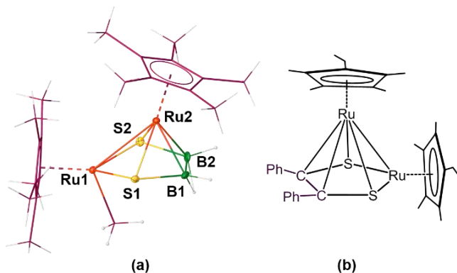
Figure 4. (a) Molecular structure and labelling diagram of 5 : Selected bond lengths (Å) and angles (°) are: Ru1-B1 2.111(13), Ru1-B2 2.188(10), Ru2-B1 2.129(12), Ru2-B2 2.180(10), Ru1-Ru2 2.6388(10), Ru1-S2 2.365(3), C21-S1 1.781(10), C21-S2 1.790(9), B1-S3 1.798(13), B2-S1 1.849(11); S1-C21-S2 113.4(5), Ru1-B1-Ru2 77.0(4). (b) schematic representation of [(\text{Cp}^*\text{Ru})_2\text{S}_2\text{C}_2\text{Ph}_2] .
