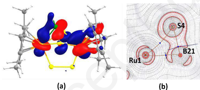
Figure 7. (a) HOMO-1 of 7 . (b) Laplacian electron density plot of 7 along Ru1-B21-S4 plane.
