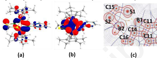
Figure 2. (a) HOMO and (b) HOMO-11 of the boryl borylene species 2 . (c) Laplacian electron density plot of the plane perpendicular to Ru-Ru bond; Solid red lines indicate areas of charge concentration ( \nabla^2\rho(r) < 0 ), while dashed black lines show areas of charge depletion ( \nabla^2\rho(r) > 0 ). Blue dots indicate bond critical points [BCPs].
