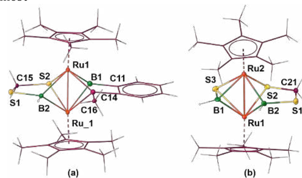
Figure 1. Molecular structure and labelling diagram of 2 (a) and 4 (b): Selected bond lengths (Å) and angles ( ^\circ ) are: 2 : C16-C14 1.526(19), B1-C11 1.575(19), C15-S1 1.73(2), C15-S2
