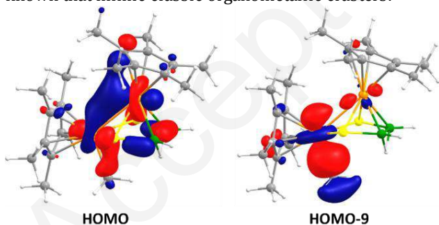
Figure 5. Selected frontier molecular orbitals of nido-5 .
