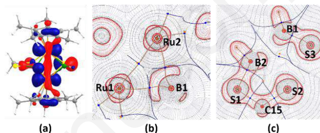
Figure 3. (a) HOMO-3 of 4 ; (b) and (c) Laplacian electron density plot of 4 of plane (Ru1-B1-Ru2) and plane perpendicular to Ru-Ru bond, respectively.
