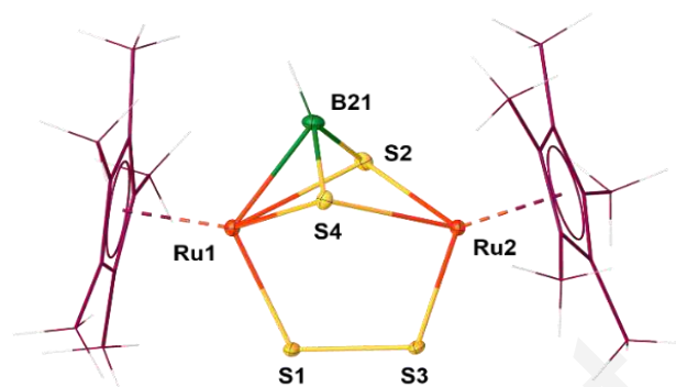
Figure 6. Molecular structure and labelling diagram of 7 . Selected bond lengths (Å) and angles (°) are: Ru1-S1 2.2599(6), Ru1-B21 2.284(3), Ru1-S4 2.4655(6), Ru2-S3 2.1916(6), Ru2-S2 2.4341(6), S1-S3 1.9985(9), B21-S2 1.809(3), B21-S4 1.826(3); S2-B21-S4 105.76(16), S2-B21-Ru1 73.28(10).
