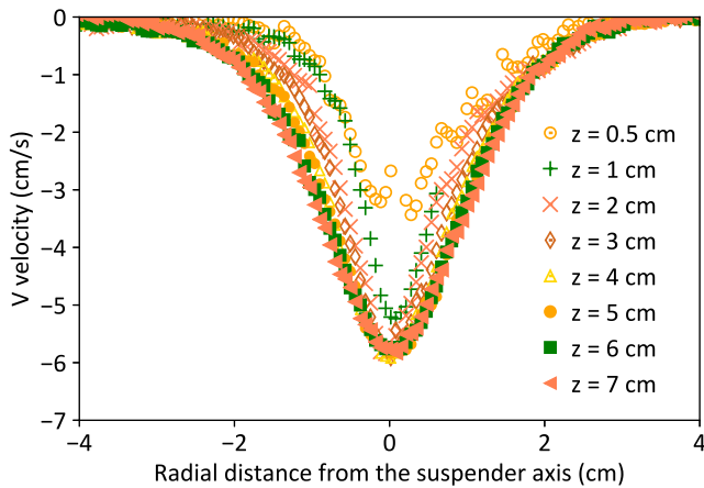
FIG. 5. Comparison of V velocity (vertical component) profiles plotted at different vertical locations ( z ) below the tip of the suspender (for ethanol evaporating in nitrogen gas). z = 0 represents the tip of the suspender.
