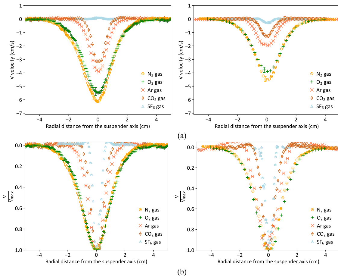
FIG. 6. (a) Comparison of velocity (vertical component) variation with distance from the axis of the suspender for evaporating ethanol (left) and water (right) droplets in different ambient gases. (b) Data as in (a) above, nondimensionalized with V_{max} . For the ethanol droplet evaporating in \text{SF}_6 , the curve has been inverted.
