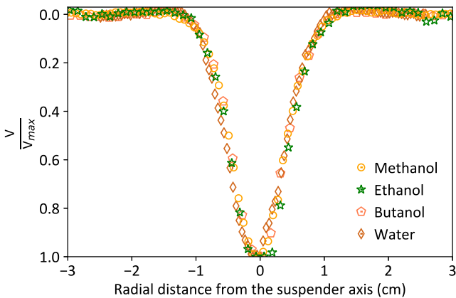
FIG. 10. Comparison of the velocity (scaled with V_{max} ) profiles due to different liquids evaporating in CO 2 ambient gas.
