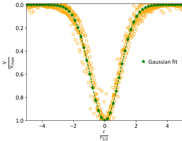
FIG. 7. Self-similarity in the flow due to the evaporating ethanol and water droplets in different ambient gases ( r_{1/2} is the radial distance at which the velocity becomes half of V_{max} ).
