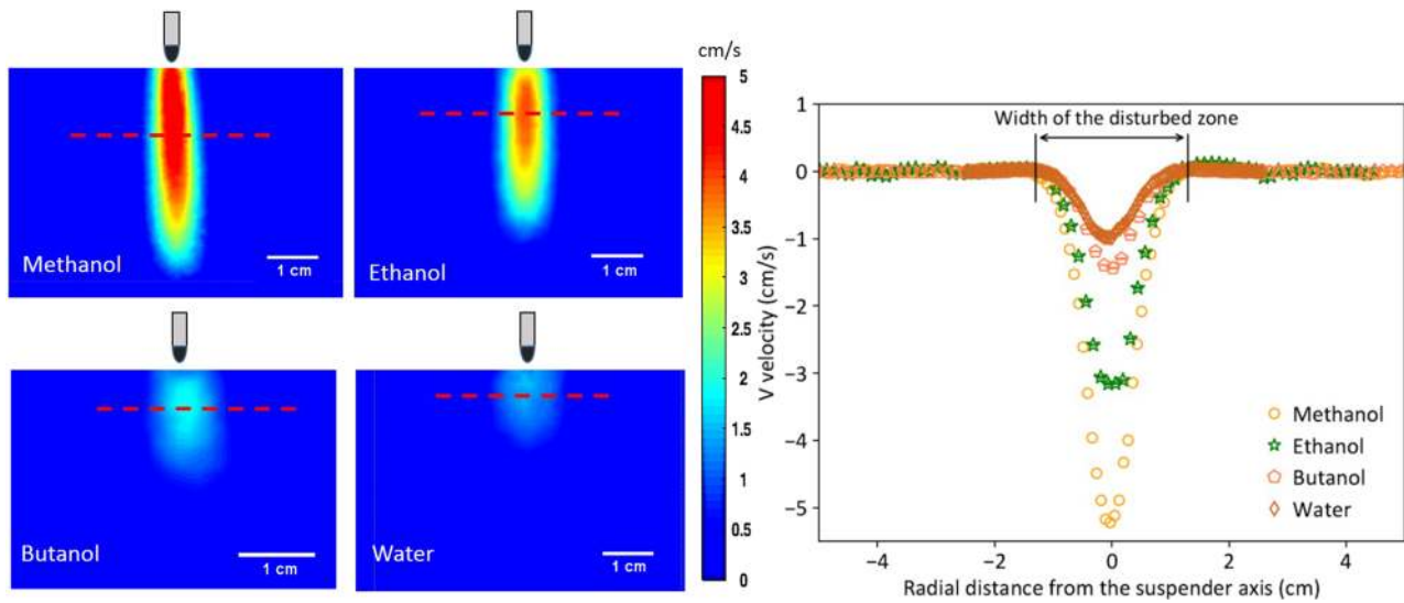
FIG. 9. Velocity contours due to different liquids evaporating in CO 2 gas are shown in the figure on the left. The suspended droplet shown in each case is just a representation and is not to scale. The figure on the right shows a comparison of the velocity (vertical) profiles corresponding to the location marked by the red dashed line (in the fully developed region) in the figure on the left.
