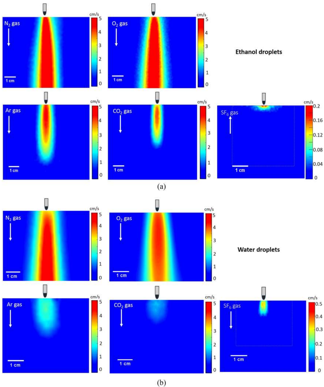
FIG. 4. Comparison of the velocity magnitudes of the flow induced around an evaporating (a) ethanol and (b) water droplet, in different ambient gases. The arrow indicates the direction of the flow. The suspended droplet shown in each case is merely a representation and is not to scale. Note: The color bar is different for SF 6 . Multimedia views: https://doi.org/10.1063/1.5109048.1 ; https://doi.org/10.1063/1.5109048.2
