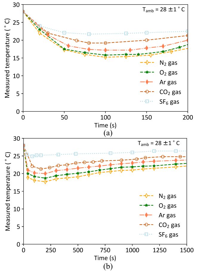
FIG. 3. Comparison of the measured surface temperature of (a) ethanol and (b) water droplets evaporating in the different ambient gases with time.
