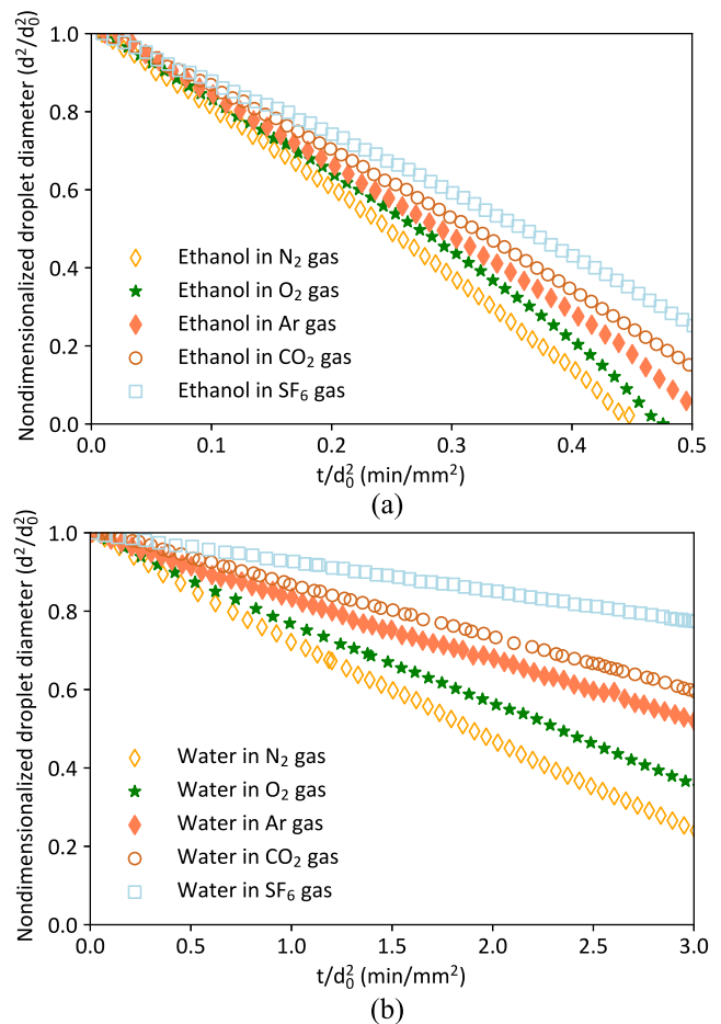
FIG. 2. Variation of the square of nondimensionalized droplet diameter with time for evaporating droplets of (a) ethanol and (b) water in different ambient gases ( d_0 is the initial droplet diameter).
