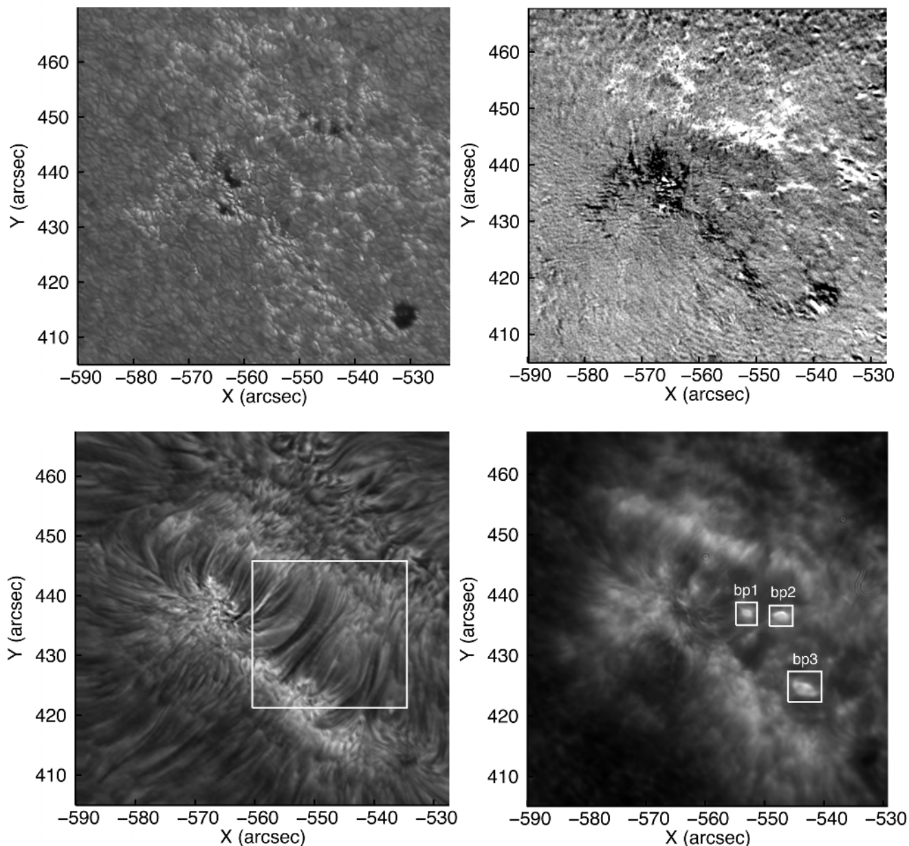
Fig. 1. Simultaneous ROSA images of the G band ( top left ), line-of-sight magnetogram ( top right ), H\alpha core ( bottom left ), and Ca II K core ( bottom right ). The magnetogram colour scale is in Gauss, where white indicates positive magnetic polarities, while black demonstrates polarities which are negative. Artificial saturation at \pm 400 G is implemented to highlight regions of weak magnetic polarity on the solar surface. The white rectangle in the H\alpha core image indicates the approximate position where most of the jets are observed. White rectangles in the Ca II K image, identified by “bp1”, “bp2”, and “bp3”, are the bright points selected for temporal analysis. Axes are in heliocentric arcseconds, where 1'' \approx 725 km.
