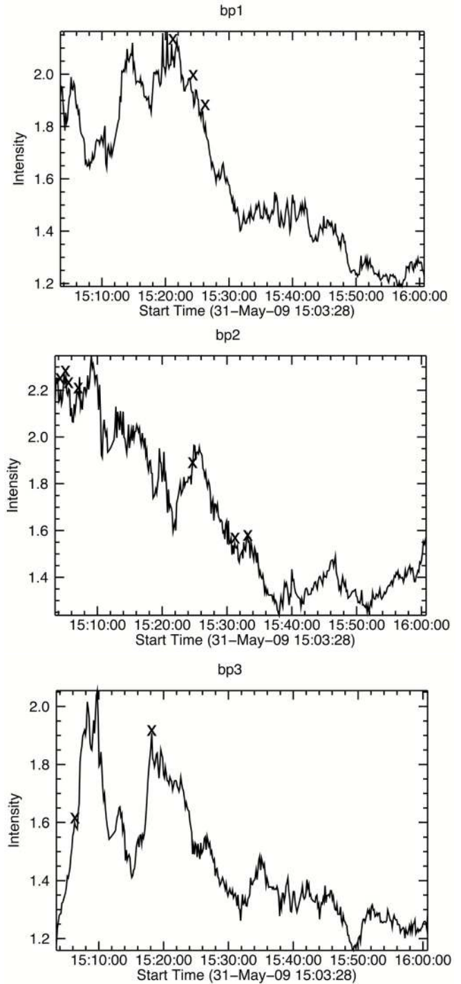
Fig. 5. Light curves of the \text{Ca II K} bright points outlined with rectangles in the lower right panel of Fig. 1. “x” symbols indicate the time when a jet event originated from that particular bright point.
