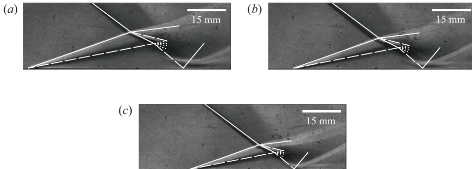
Figure 17. Separation bubble geometry between the experiments and the LESF model at shock impingement locations (a) X_{ir} \approx 60 mm, (b) X_{ir} \approx 50 mm and (c) X_{ir} \approx 40 mm. The figures clearly show a geometric similarity of the SWBLI at different shock impingements. The LESF model agrees well with the experiments. The shock wave, slip line and expansion fan of the LESF model are denoted by continuous, dashed and dotted lines, respectively. The model assumes \kappa = 1 . For all cases in the figure, M_\infty = 5.52 , \theta_w = 26.6^\circ .
