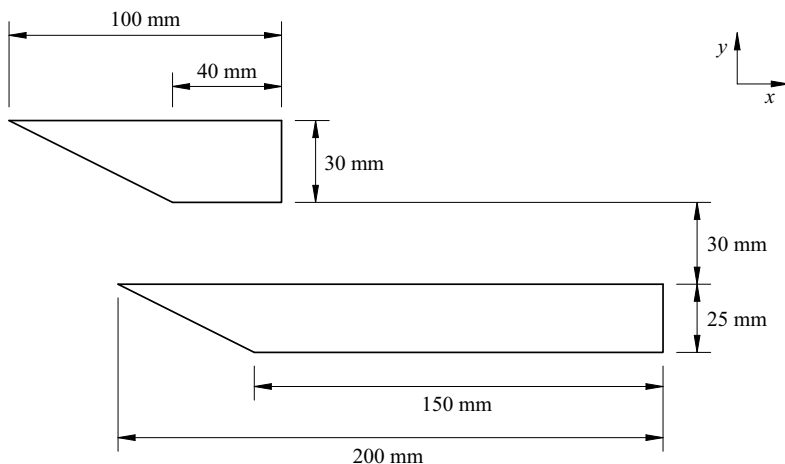
Figure 6. Two-dimensional drawing of a typical model arrangement. Wedge (top) and plate wall (bottom) are the test models used, each having a span of 120 mm (not shown in the figure).
