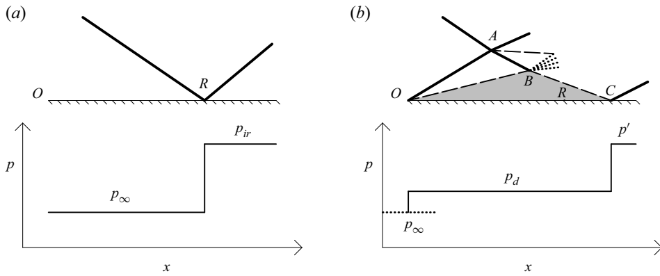
Figure 9. Schematic diagram (not to scale) and wall pressure profiles of (a) unseparated and (b) separated flows. The unseparated flow is characterized by the pressure jump p_{ir}/p_\infty and the shock impingement distance X_{ir} = OR . The separated flow is characterized by the pressure jumps p_d/p_\infty and p'/p_d , and the separation length L = OC .
