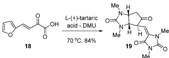
Scheme 3 Unusual formation of a bicyclic alkyldine hydantoin derivative.
