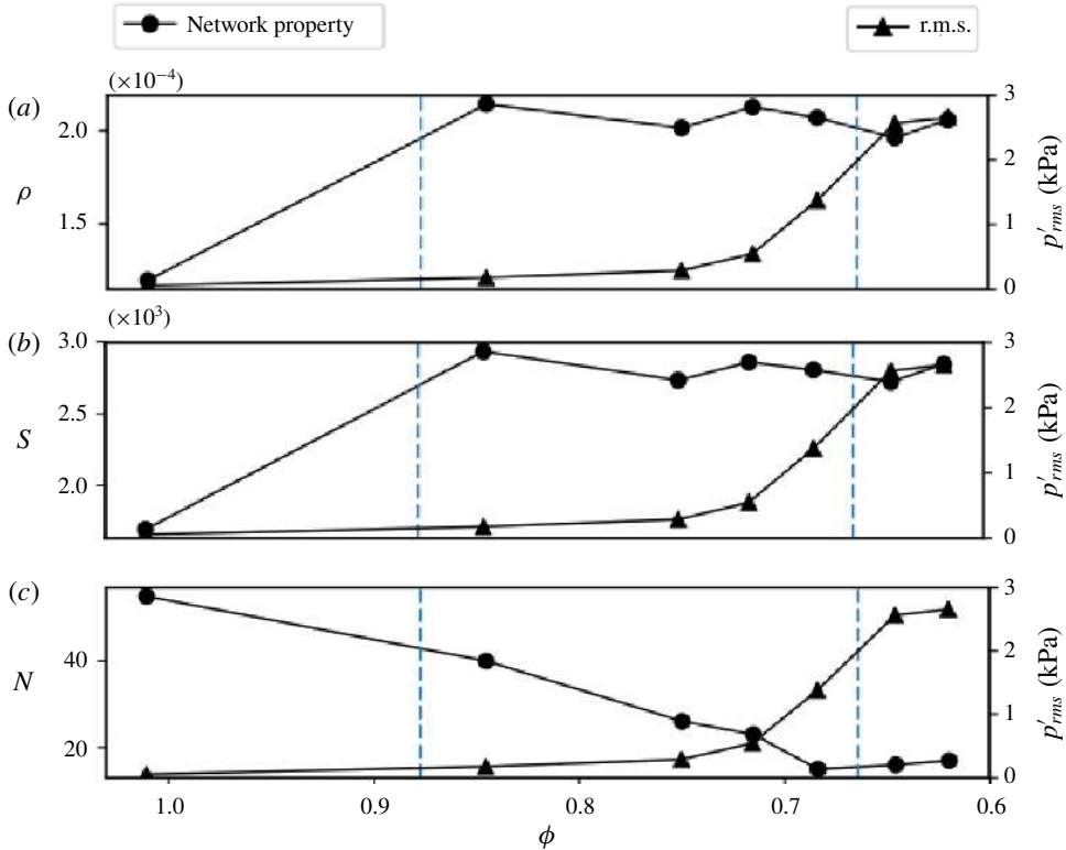
FIGURE 11. (Colour online) Variation of the standard deviation of the network properties: (a) the link density ( \rho ), (b) the size of the giant cluster ( S ) and (c) the number of clusters ( N ), along with the variation of the r.m.s. value of the acoustic pressure as the thermoacoustic system transits from combustion noise to thermoacoustic instability via intermittency. The dashed vertical lines divide the parameter space, i.e. the equivalence ratio ( \phi ), into regimes of combustion noise, intermittency and thermoacoustic instability, respectively.
