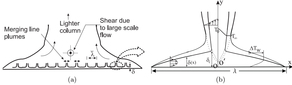
FIGURE 7. A schematic of the assumed phenomenology for the analysis. (a), Merging line plumes near the wall result in rising lighter column of fluid that drives the large scale flow. The large scale flow causes shear in the direction perpendicular to the plane of the figure thereby aligning the line plumes. (b), The magnified view of the region marked with a dashed ellipse in (a). Two natural convection boundary layers become unstable at a critical distance of \bar{\lambda}/2 when \delta(x) = \delta_c to give rise to a line plume. O' is the virtual origin of the plume.
