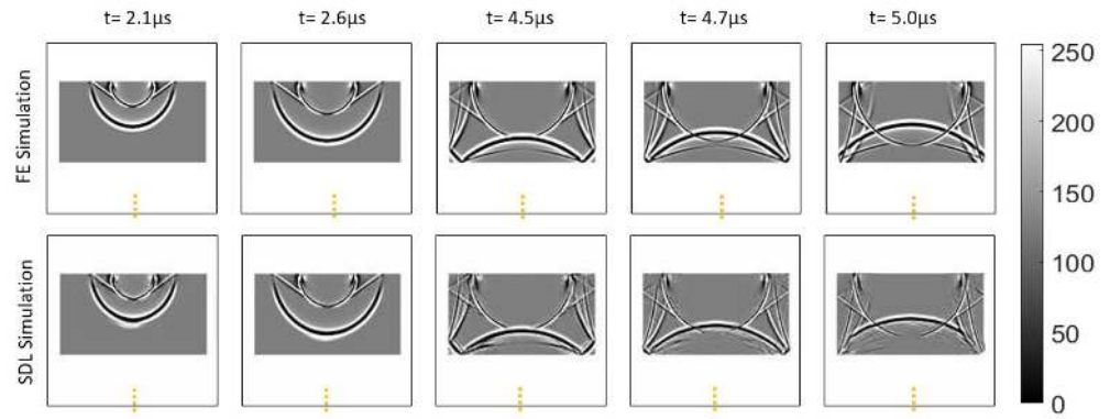
(a) FE/SDL simulation comparison for the 4 MHz central frequency, with two cycles.
