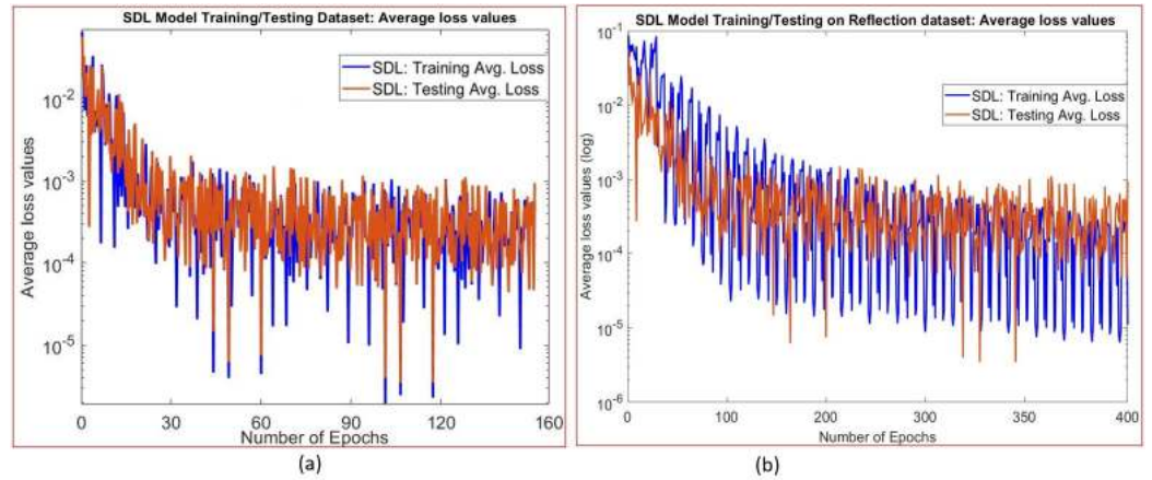
Figure 3. (a) Spatio-temporal deep learning (SDL) model, for forward wave propagation: training and testing average loss values over the number of epochs for the type-1 datasets. (b) Spatio-temporal deep learning (SDL) model, for reflected wave propagation: training and testing average loss values over the number of epochs for the type-2 datasets.
