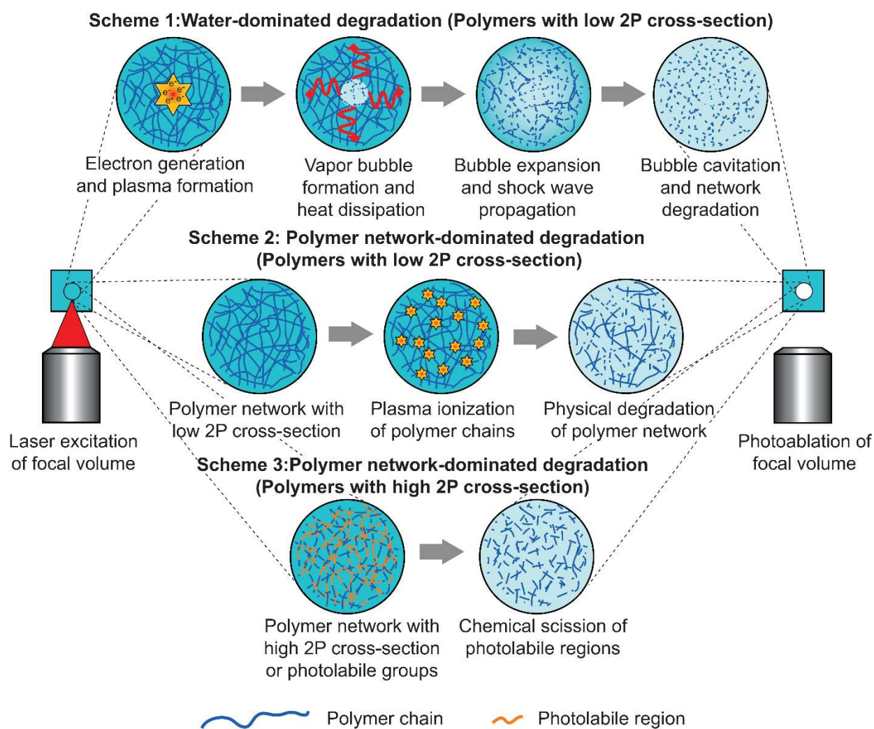
Figure 6. Schematic of the various modes of laser-hydrogel interactions. Laser-induced degradation of hydrogels can follow various modes depending on the type and composition of polymeric material. Scheme 1: the water within the polymeric network is excited by the laser and undergoes electron generation, plasma formation, and vapor bubble generation. The vapor bubble expands radially along with shock wave propagation and heat dissipation and subsequently causes physical breakage of the network due to thermoelastic stress. Scheme 2: the polymeric network is excited by the incident laser light and undergoes plasma formation which subsequently leads to physical breakage of polymer network. Scheme 3: hydrogels with a high two-photon cross-section or those containing photolabile groups undergo direct chemical scission which induces rapid dissociation of the polymer network.
