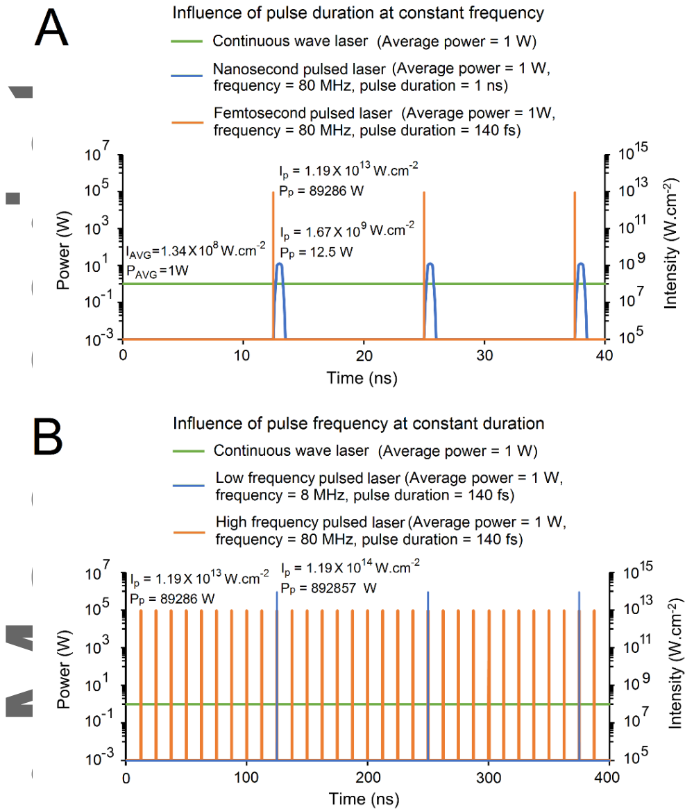
Figure 2. Theoretical power and intensity outputs for three different lasers over time as a function of pulse duration and pulse frequency. A) Comparison of the power and intensity over time for three different lasers (continuous wave, 1 ns pulsed, and 140 fs pulsed) operating at the same pulse frequency for the pulsed lasers (80 MHz), same average power (1 W), and same average intensity ( 1.34 \times 10^8 \text{ W cm}^{-2} ) but with different pulse durations, 1 ns and 140 fs for the pulsed lasers. The fs-pulsed laser outputs a higher peak power and intensity compared to the ns-pulsed or continuous-wave lasers to achieve the same average power and intensity. B) Comparison of the power and intensity output over time for three different lasers (continuous wave, low-frequency (8 MHz) fs pulsed, and high-frequency (80 MHz) fs pulsed) operating at the same average power (1 W) and same average intensity ( 1.34 \times 10^8 \text{ W cm}^{-2} ) with the same pulse duration for the pulsed lasers (140 fs) but at different frequencies. The laser operating at the lower frequency (8 MHz) outputs a higher peak power and intensity to achieve the same average output compared to the higher frequency pulse and continuous wave lasers. ( I_p : peak intensity, P_p : peak power, I_{AVG} : average intensity, P_{AVG} : average power).
