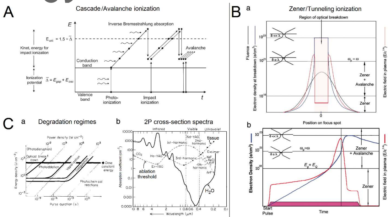
Figure 3. Interplay of physical mechanisms influencing laser-based degradation. A) The sequential occurrence of photoionization, inverse Bremsstrahlung absorption, and impact ionization leads to plasma formation and recurring sequences in absorption and ionization events lead to avalanche growth of free electrons produced by laser excitation. Reproduced with permission. [48] Copyright 2005, Springer-Verlag. B) Schematic illustration of a) distribution of processes in the focal volume and b) sequence of processes occurring over the course of a laser pulse. Zener ionization and Zener-seeded avalanche ionization cause increases in the electron density and plasma field intensity in the focal volume. The laser penetration depth ( \delta ) becomes approximately equal to the wavelength ( \lambda ) at 10^{21} electrons cm^{-3} . When plasma frequency ( \omega_p ) becomes equal to the laser frequency ( \omega ), rapid ionization and heavy absorption take place and material over depth, \delta , is vaporized. The pink region at the bottom indicates the duration of the laser pulse. E_Q and E_G refer to the electron quiver energy and
