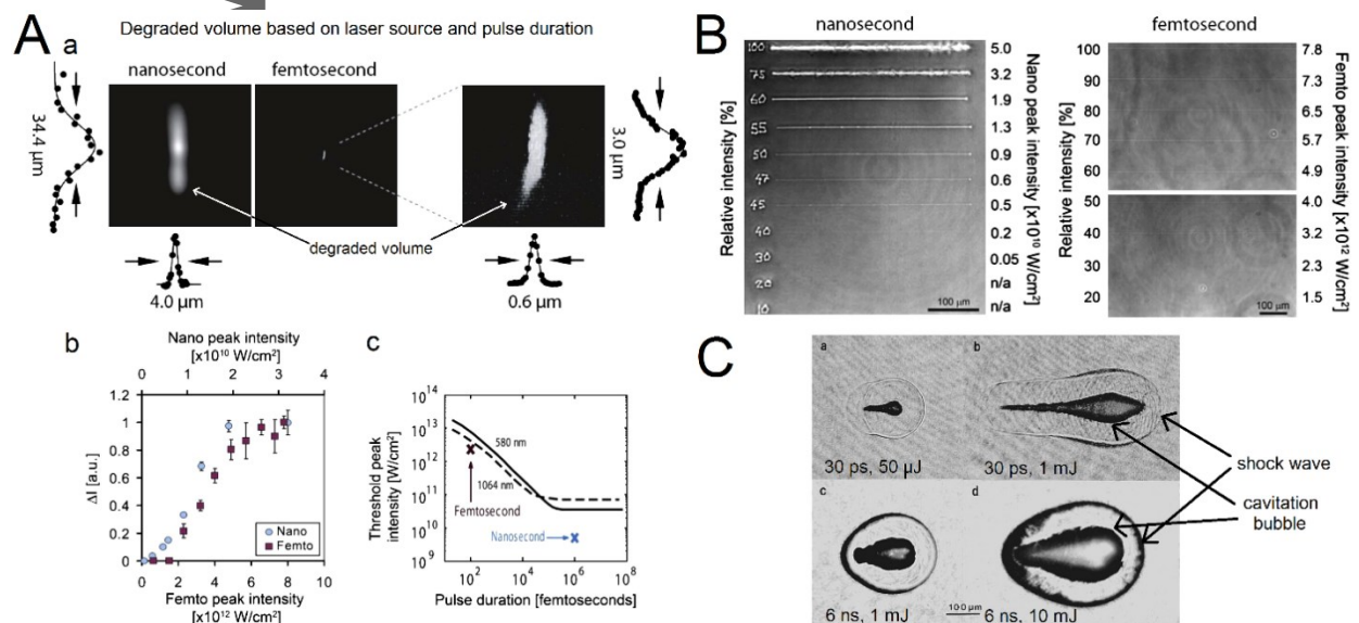
Figure 4. Effect of pulse duration on laser-material interactions. A) a) Degradation using a femtosecond pulsed laser provides increased spatial resolution compared to a nanosecond pulsed laser as demonstrated by the lateral and axial dimensions of the degradation volume. b) The visible-laser-
