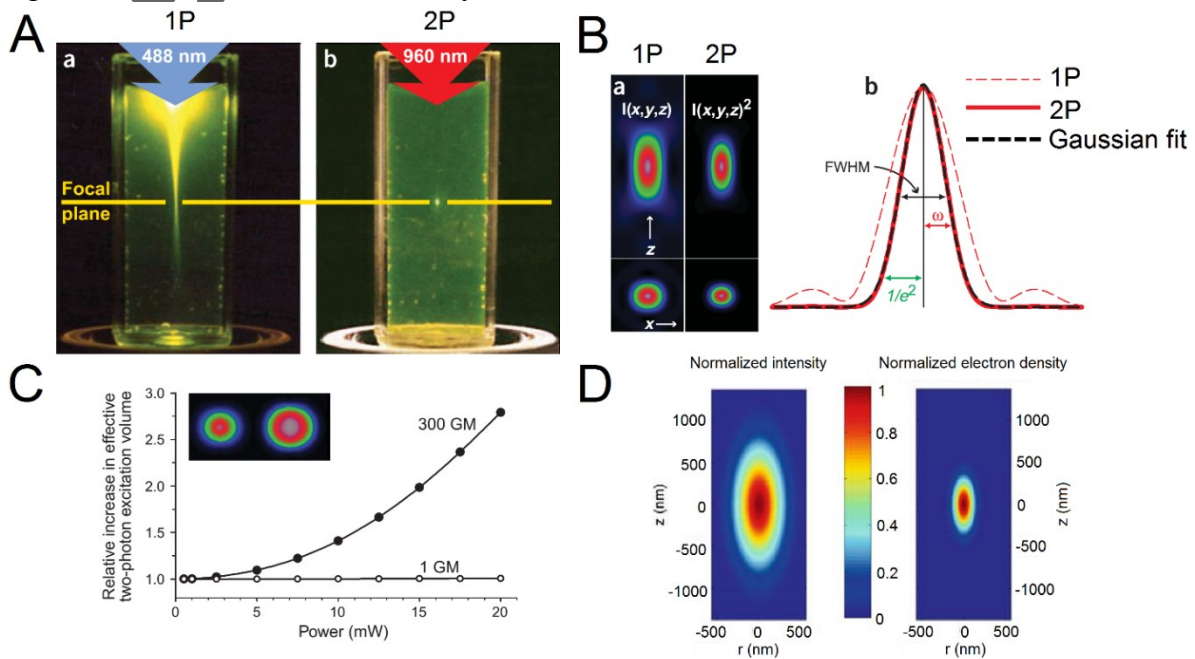
Figure 5. Characterization of the two-photon excitation volume. A) Visualization of the excitation volume for single-photon (1P) and two-photon (2P) excitation of fluorescein using a) a continuous wave laser at 488 nm and b) a femtosecond pulsed laser at 960 nm focused through a NA 0.16 objective. B) a) Lateral and axial views of the point spread function using 1P and 2P excitation. b) FWHM refers to the full-width half-maximum of the Gaussian fit and \omega refers to the axial radius. C) The 2P excitation volume calculated for a 1-GM and a 300-GM fluorophore excited using a 200 fs pulsed laser operating at 80 MHz focused through a 1.2 NA objective. Inset shows the point spread function for excitation of a 1 GM (left) and 300 GM (right) fluorophore at 20 mW. Reproduced with permission. [59] Copyright 2003, Nature Publishing Group. D) The distribution of the normalized intensity and electron density in a focal volume of a femtosecond pulsed laser during optical breakdown using a 1.3 NA objective and 800 nm light. Reproduced with permission. [48] Copyright 2005, Springer-Verlag.
