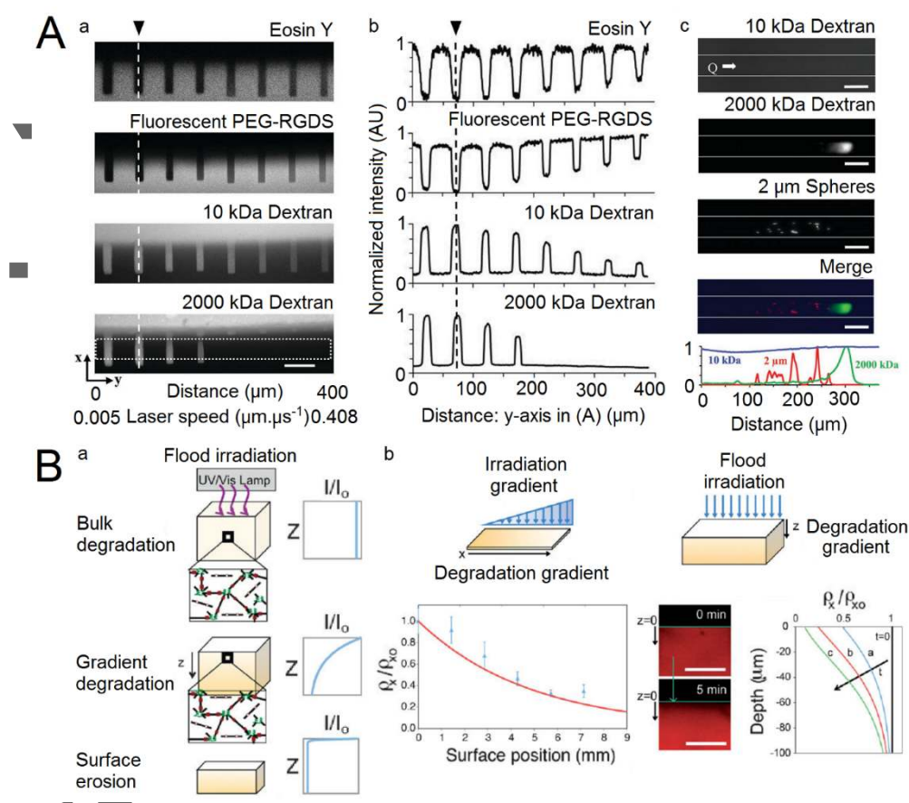
Figure 13. Controlled laser-based hydrogel degradation to spatially regulate hydrogel porosity. A) a–b) Control of hydrogel porosity through variation of the laser scan speed at constant fluence as evidenced through quantification of fluorescence intensities of Eosin Y, PEG-RGDS, and diffusion of 10 kDa and 2000 kDa dextran through the degraded channels. c) Size-based separation of fluorescent species by local control of hydrogel porosity across a linear distance under a flow rate of 10 \mu\text{l min}^{-1} and quantitative measurement of fluorescence intensities of separated species. Scale bars = 50 \mu\text{m} . Reproduced with permission. [34] B) a) Schematic of the different modes of degradation of photolabile hydrogels via flood irradiation and their corresponding attenuated intensity profile through the depth of the hydrogel. b) Induction of degradation gradients in photolabile hydrogels via gradient irradiation or via attenuation of flood irradiation through the hydrogel thickness over time (2.5, 5, or 8 min) and corresponding changes in normalized crosslinking densities. Scale bars = 100 \mu\text{m} . Reproduced with permission. [69]
