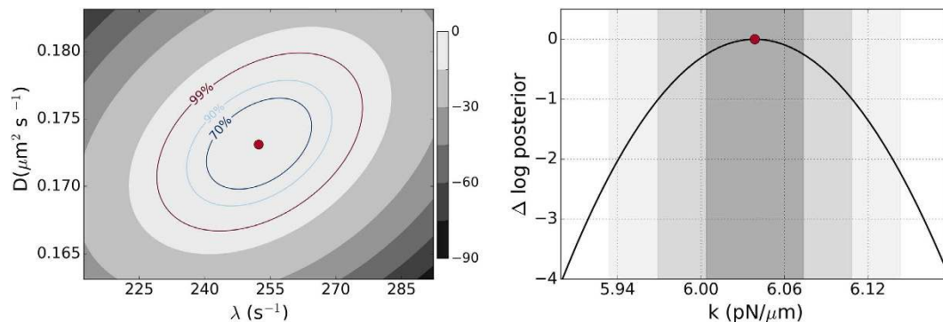
Figure 3. Bayesian posterior probability densities. The left panel shows filled contours of Eq. (11). The MAP estimate, Eq. (12), is marked by the filled dot and contours enclosing 70%, 90% and 99% of the probability are labeled. The middle panel shows Eq. (14). The MAP estimate, Eq. (15), is marked by the filled dot and intervals enclosing 70%, 90% and 99% of the probability are shaded. The two estimates for k agree to three decimal places. The analysis is for polystyrene bead of radius a = 3 \mu\text{m} .
