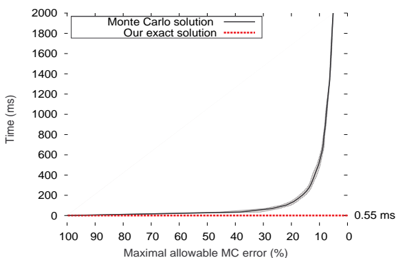
Figure 6: g_2, k = 2 , WSPG (UW)
