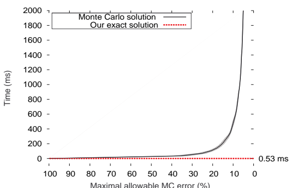
Figure 8: g_2, k_i = \frac{3}{4} deg_i , WSPG (UW)
