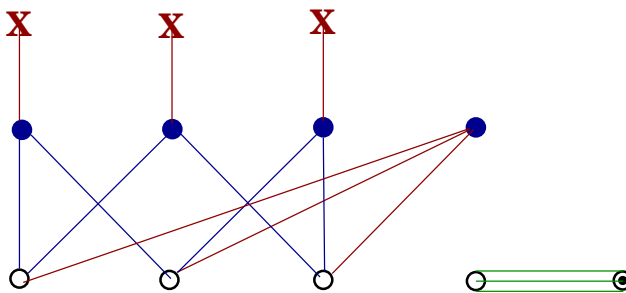
Figure 6: \mathcal{C}_{4a} = -(\frac{3}{4}a^4 + 6a)(\kappa_{123} - \kappa_{132}) .
