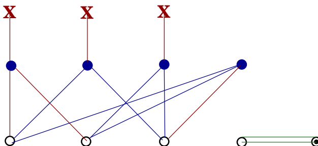
Figure 7: \mathcal{C}_{4b} = -(\frac{3}{4}a^4 + 6a)(\kappa_{123} - \kappa_{132}) .
