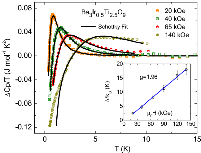
FIG. 5. A few representative plots of [C_P(H) - C_P(H = 0)]/T or (\Delta C_P/T) for \text{Ba}_3\text{Ir}_{0.5}\text{Ti}_{2.5}\text{O}_9 at various values of the field H (as given in the legend) and their fit to Eq. (1) (black lines). (Inset) Variation of the Schottky gap as a function of magnetic field for orphan spins.
