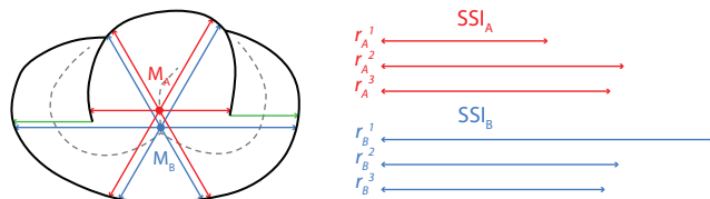
Fig. 6. Example of SSI for points M_A (resp. M_B ) constructed by measuring the local reaches r_A^k (resp. r_B^k ) in the k th direction of a uniformly sampled set of m directions (here m = 3 ). Some discontinuities of reach are present and shown here as green arrows.
