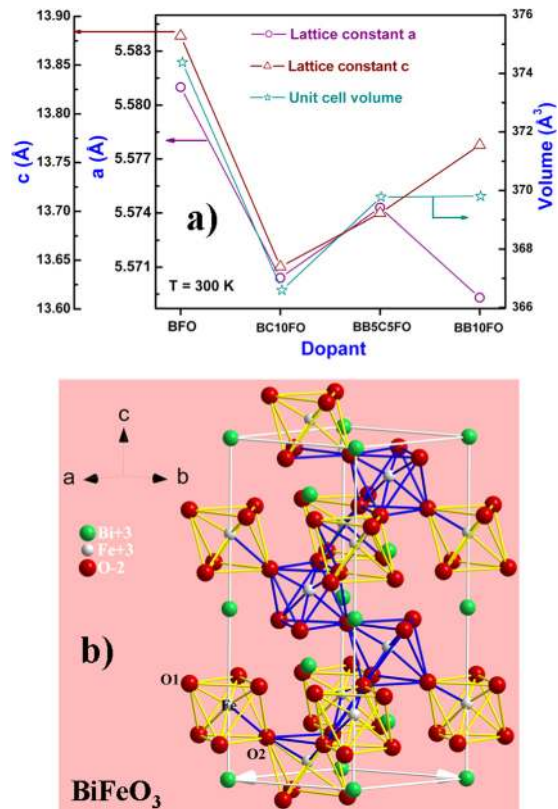
FIG. 2. (Color online) (a) Lattice constants and unit cell volume vs dopant and (b) crystal structure of BiFeO 3 . Blue and yellow color bonds represent bonds that are inside and outside of the unit cell in the Fe-O octahedra, respectively.
