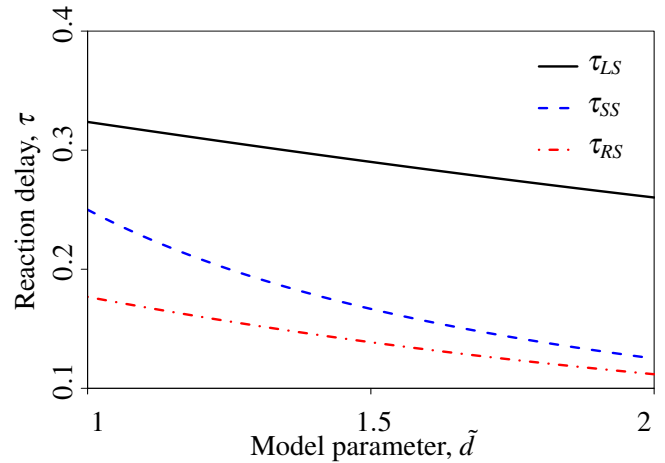
Fig. 1. Stability chart: Diagram depicting the boundaries of local pairwise stability ( \tau_{LS} ), string stability ( \tau_{SS} ) and pairwise robust stability ( \tau_{RS} ) for the MOVIM.
