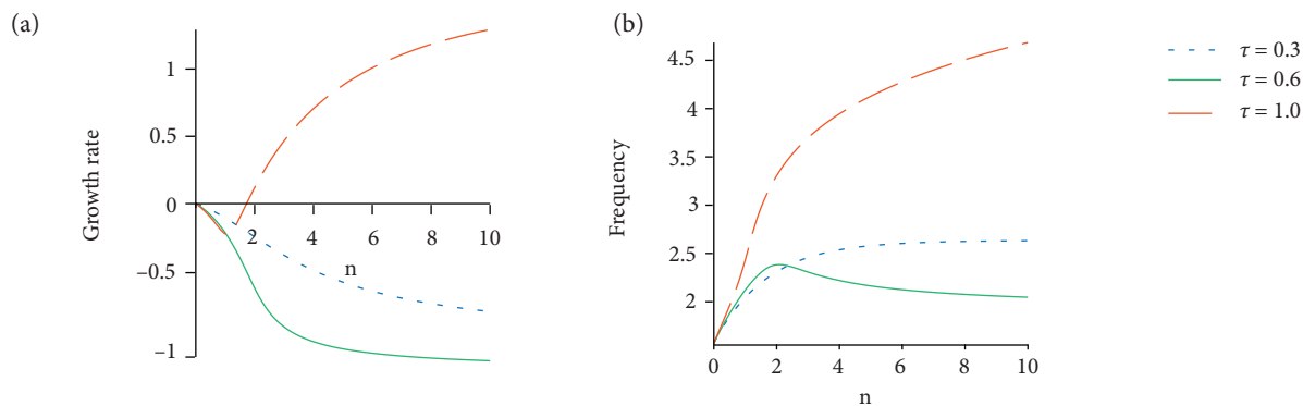
Figure 5. Thermoacoustic characteristics of a duct (1L mode, x_f = 0.10 ) showing (a) growth rate and (b) frequency.
