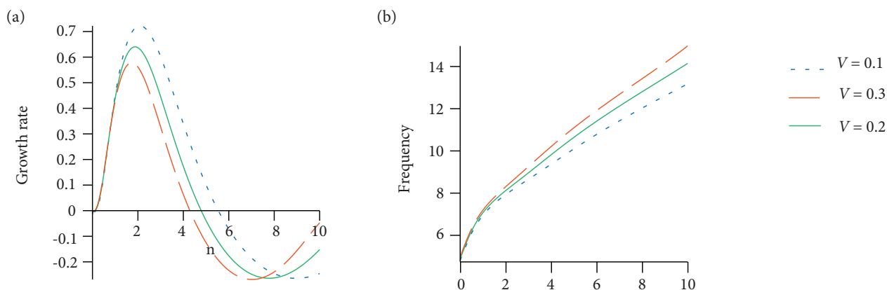
Figure 16. Thermoacoustic characteristics of a ducted resonator as volume ratio varies [3L mode, \tau = 0.6 , x_f = 0.10 , x_h = 0.5 , \omega_h = 2 ] showing (a) growth rate and (b) frequency.
