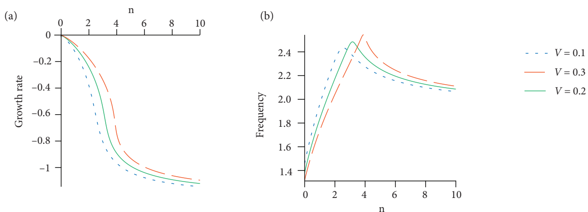
Figure 15. Thermoacoustic characteristics of a ducted resonator as volume ratio varies [1L mode, \tau = 0.6 , x_f = 0.10 , x_h = 0.5 , \omega_h = 2 ] showing (a) growth rate and (b) frequency.
