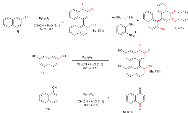
Scheme 6 Synthesis of substituted naphthoquinones
