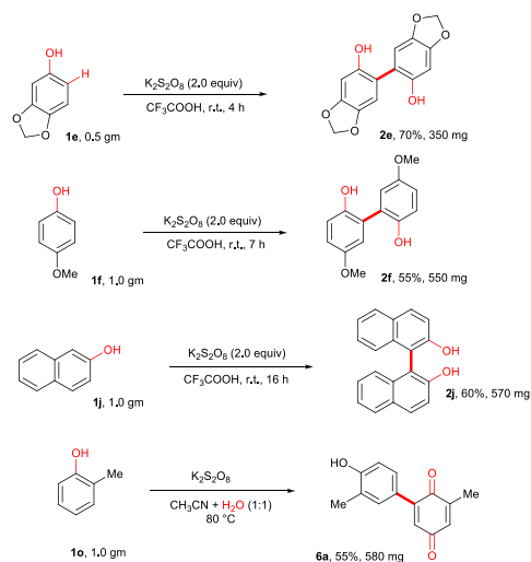
Scheme 7 A gram scale synthesis of biphenols
