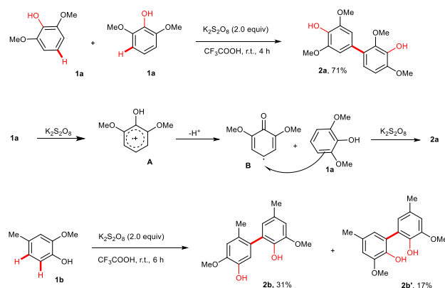
Scheme 1 Cross-coupling of phenols 1a-b
