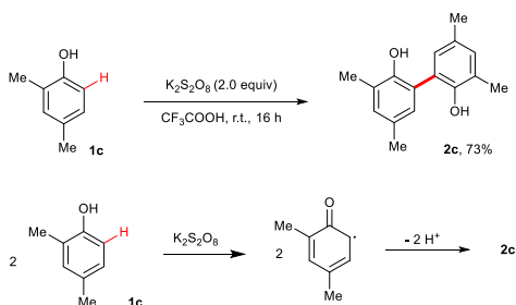
Scheme 2 Homocoupling of 2,4-dimethylphenol ( 1c )
