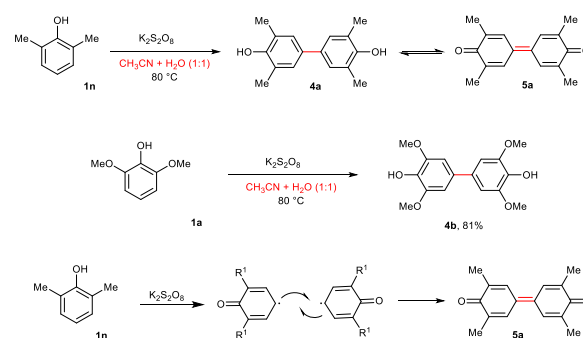
Scheme 4 para-para Coupling of phenols
