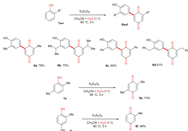
Scheme 5 Synthesis of substituted benzoquinones
