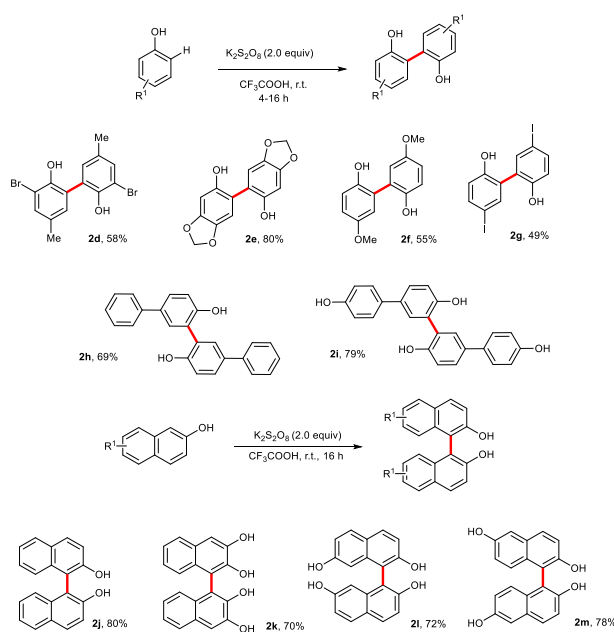
Scheme 3 Scope of phenols and naphthols
