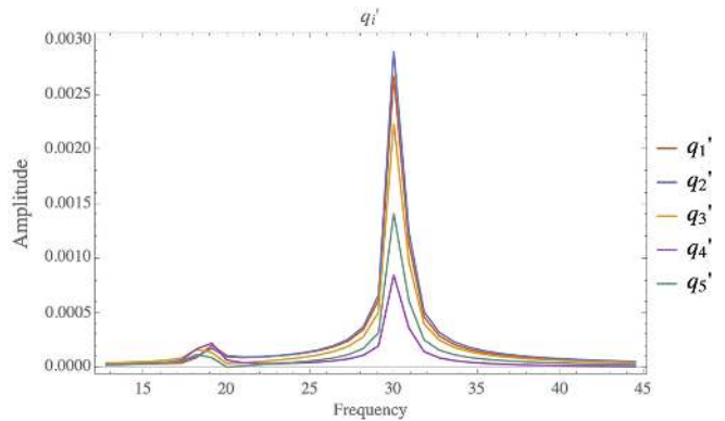
FIG. 7. Amplitudes of the Fourier transform of q_i' for each site obtained after the full system relaxes to the final microstate. The peaks coincide with the numerically computed normal mode frequencies to a very good approximation. The finite width of these peaks is due to finiteness of the time window and also numerical noise.
