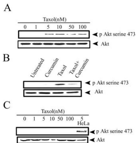
FIG. 6. Taxol-induced Akt activation is down-regulated by curcumin in HeLa cells, whereas normal cells remain unaffected. A , HeLa cells were treated with Taxol (0–100 nM) for 1 h, and the whole cell lysate was resolved on 10% gel and blotted against phospho-Akt serine 473. B , HeLa cells were treated with Taxol (5 nM) and/or curcumin (5 \mu M) for 1 h, and the whole cell lysate was resolved on a 10% gel and blotted against phospho-Akt serine 473. C , normal cervical cells were treated with Taxol (0–100 nM) for 1 h, and whole cell lysate was resolved on a 10% gel and blotted against phospho-Akt serine 473. Cell lysates of HeLa cells treated with 5 nM Taxol were loaded as a positive control.
