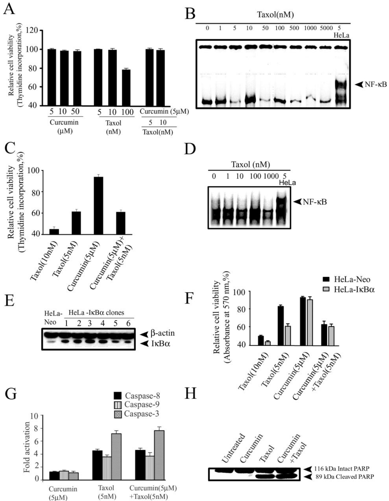
FIG. 5. Curcumin does not sensitize Taxol-induced apoptosis in normal cervical cells, human 293 cells, or HeLa-I \kappa B \alpha cells. A , normal cervical cells were treated with Taxol and/or curcumin as indicated for 24 h, and [ ^3 H]thymidine incorporation was determined as described under "Experimental Procedures." B , normal cervical cells were treated with Taxol (0–5000 nM), nuclear extracts were prepared, and EMSA was done as described under "Experimental Procedures." The nuclear extracts of HeLa cells treated with 5 nM Taxol were loaded as a positive control. C , human 293 cells were treated with Taxol and/or curcumin as indicated for 24 h, and [ ^3 H]thymidine incorporation was determined as described under "Experimental Procedures." D , human 293 cells were treated with Taxol (0–1000 nM), nuclear extracts were prepared, and EMSA was done as described under "Experimental Procedures." Nuclear extracts of HeLa cells treated with 5 nM Taxol were loaded as a positive control. E , HeLa cells were transfected with pcDNA3 vector or the pcDNA3-I \kappa B \alpha construct using a calcium phosphate transfection kit, and the G418-resistant clones were selected as described under "Experimental Procedures." Cell lysates from the vector-transfected HeLa-Neo cells and the different clones of HeLa-I \kappa B \alpha cells were immunoblotted for I \kappa B \alpha and \beta -actin. F , HeLa-Neo and HeLa-I \kappa B \alpha cells were treated with Taxol and/or curcumin
