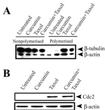
FIG. 7. Sensitization of Taxol-induced apoptosis by curcumin is independent of tubulin polymerization and cell cycle arrest. A , HeLa cells were treated with Taxol (5 nM) and/or curcumin (5 \mu M) for 24 h, and polymerized and non-polymerized tubulin were isolated as described under “Experimental Procedures” and resolved on a 10% gel and blotted against anti- \beta -tubulin and anti- \beta -actin. B , HeLa cells were treated with Taxol (5 nM) and/or curcumin (5 \mu M) for 1 h, and whole cell lysate was resolved on a 10% gel and blotted against anti-Cdc2.
