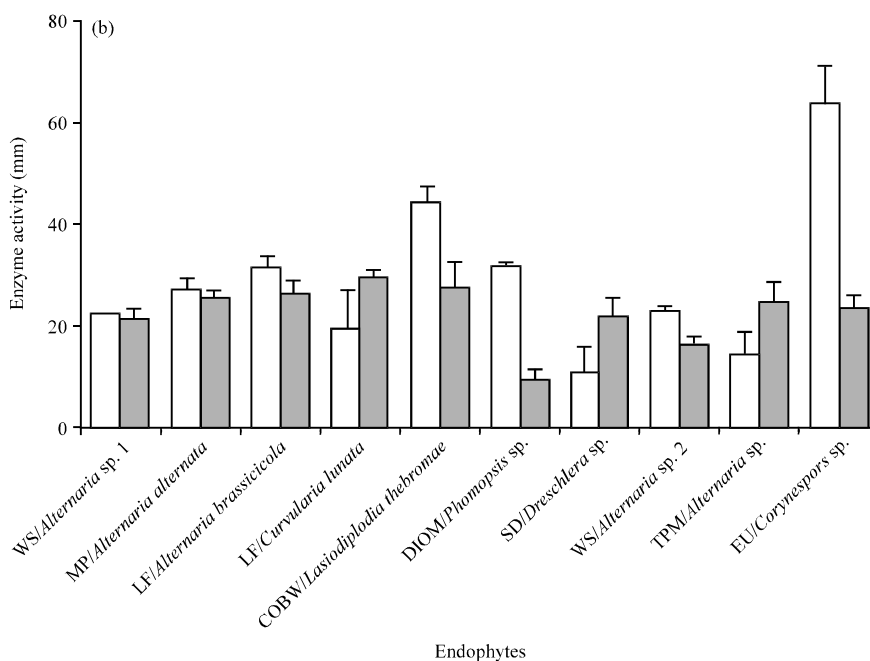
Fig. 3(a-b): Effect of glucose on (a) Colony growth and (b) Enzyme activity by plate assay in L-asparaginase producing fungal endophytes. There is a significant decline in L-asparaginase activity of DIOM/ Phomopsis sp., WS/ Alternaria sp., 2 and EU/ Corynespora sp. in the presence of glucose ( p < 0.05 , by ANOVA). In WS/ Alternaria sp. 1, Alternaria alternata and WS/ Alternaria brassicicola , the mean colony growth decreases significantly ( p < 0.05 , by ANOVA) in the presence of glucose. Experiment was repeated thrice and the error bars represent standard error of mean
