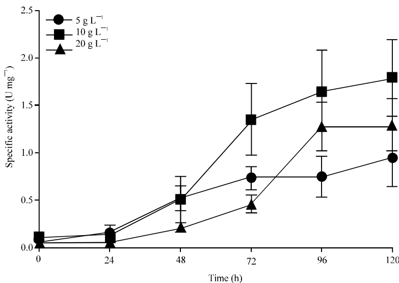
Fig. 6: Effect of L-asparagine on specific activity of glutaminase free L- aspariginase in shake flask at varying concentrations of L-asparagine 5, 10 and 20 g L -1 . Experiment was repeated thrice and the error bars represent standard error of mean
