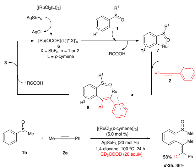
Scheme 1 Proposed mechanism
