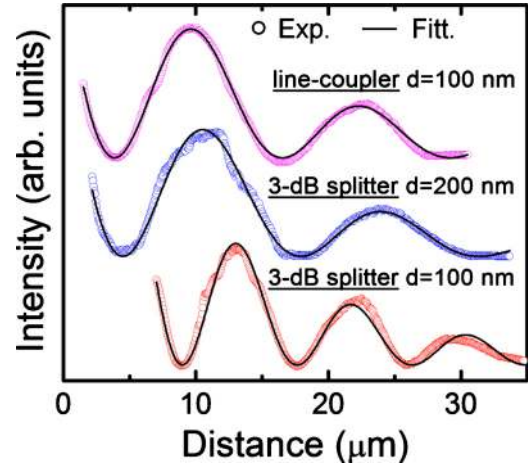
FIG. 2. (Color online) Line profiles and fittings to the data using Eq. (1) of the line-coupler ( d=100 nm) and 3 dB splitters ( d=100 nm and d=200 nm) shown in Figs. 1(b) and 1(d), respectively.
