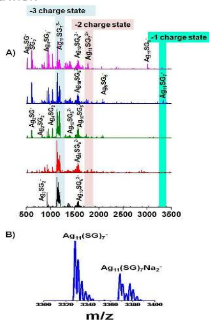
Figure 3: A) SID of \text{Ag}_{11}(\text{SG})_7\text{Na}_3^{3-} at increased voltage shows multiple fragmentations at all the energies, unlike in CID. At higher voltages, charge stripping was observed to give a -2 charged species and finally at SID 40, -1 ion peak was observed. Two Na attached peaks were also observed as expanded in B).
