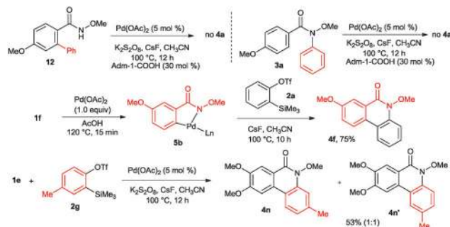
Scheme 5 Mechanistic investigation.
