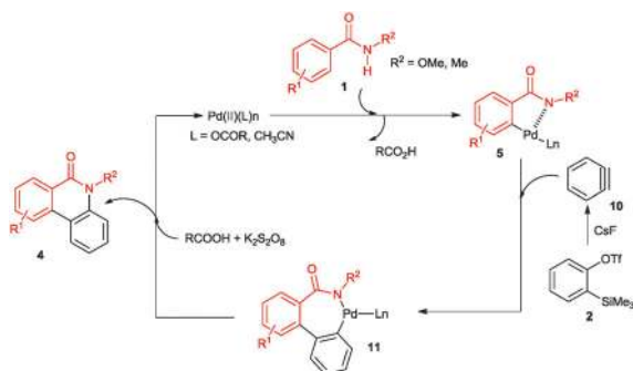
Scheme 4 Proposed mechanism.
