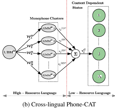
Figure 1: Cross-lingual Models
