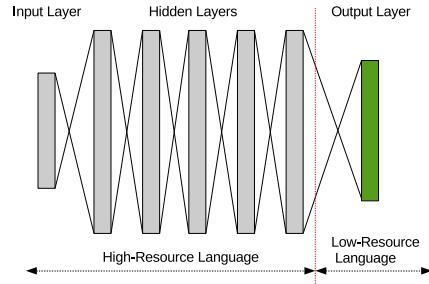
Figure 2: Cross-lingual DNN
