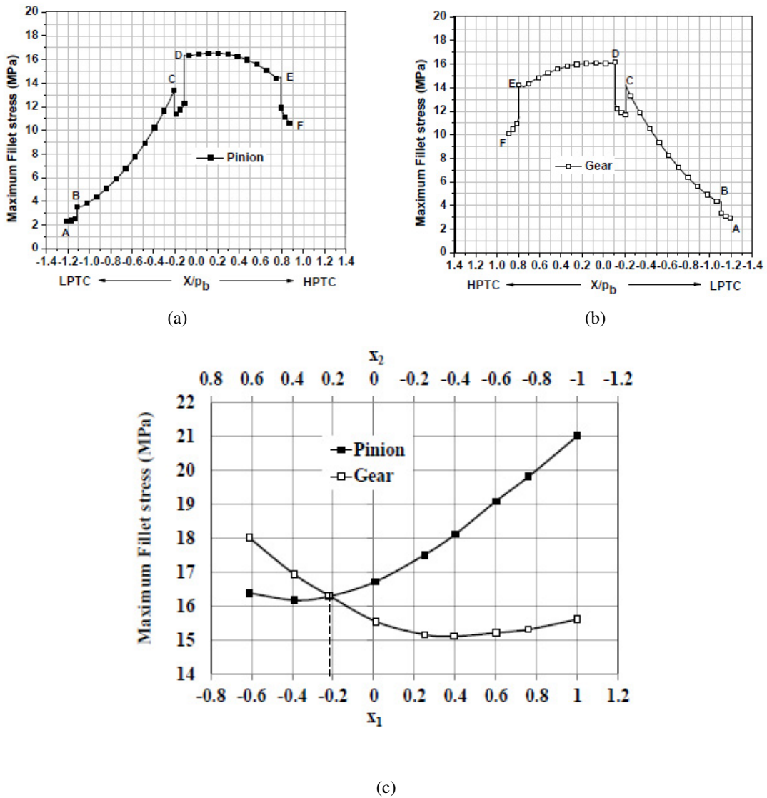
Fig. 5 Optimum profile shifts estimation based on (\sigma_t)_{max} for a load at high pressure angle side ( m=1, z_1=50, i=2, k=1.1, \epsilon_d=2.1 ). a) (\sigma_t)_{max} vs. contact position for pinion. b) (\sigma_t)_{max} vs. contact position for Gear e) (\sigma_t)_{max} vs. profile shift on pinion and gear.
