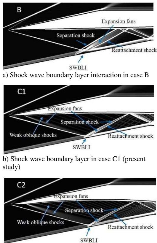
a) Shock wave boundary layer interaction in case B b) Shock wave boundary layer in case C1 (present study) c) Shock wave boundary layer interaction in case C2 (present study) Fig. 9. Shock wave boundary layer interaction.
