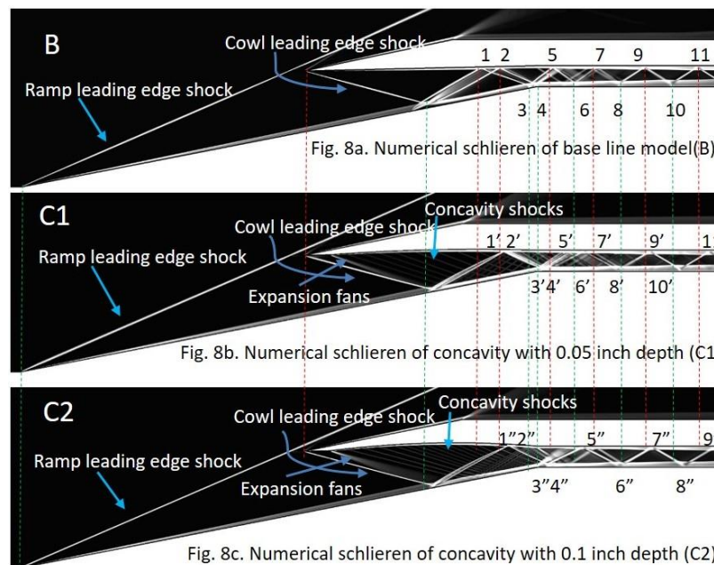
Fig. 8. Numerical schlieren of cases B, C1 and C2.
