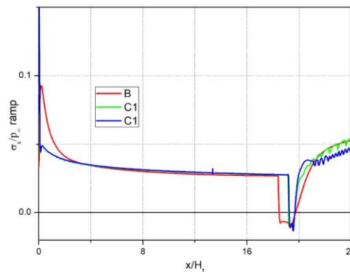
Fig. 10. Wall shear stress along the ramp surface.
