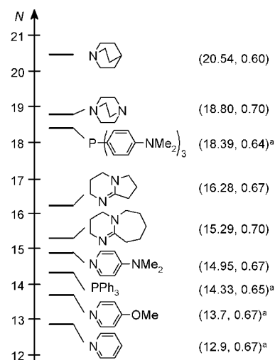
Scheme 1 Comparison of the nucleophile specific reactivity parameters ( N , s ) for different organocatalysts in acetonitrile. a N parameters refer to CH 2 Cl 2 .
