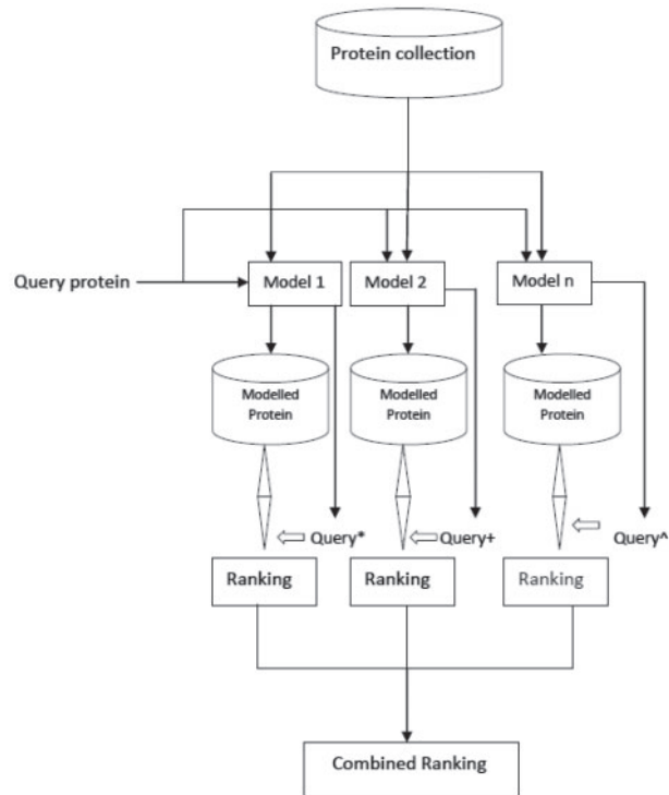
Fig. 4. Multi-viewpoint-based IR.
