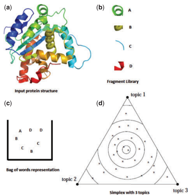
Fig. 2. Example protein structure with bag of fragments and topic space representations; built for a given fragment library. (a) shows an example protein structure and (b) shows a given fragment library. Each substructure in protein is compared against the fragment library and the closest matching fragment is used to represent the substructure. Thus, we obtain bag of fragments representation for protein structure as shown in (c). We model the structure as a probability distribution over latent topics. In (d) we have shown a toy representation using three topics, which forms a simplex.
