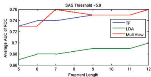
Fig. 8. Comparison of the average AUC at SAS threshold of 5.0 Å, across libraries, obtained using TF, LDA and multiview model using the best weights from Table 5.
