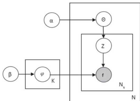
Fig. 1. Graphical representation of LDA; K is the number of topics; N is the number of protein structures; N_s is the number of fragments in protein structure s .
