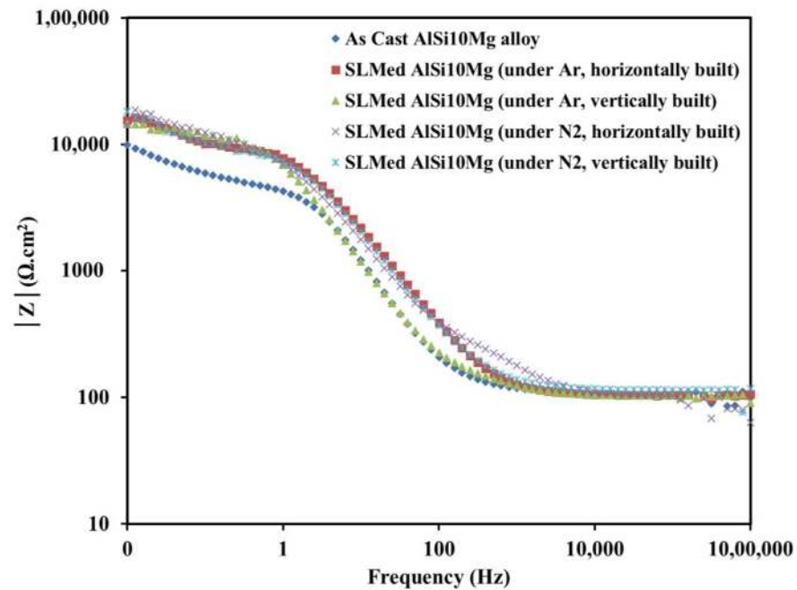
Figure 10. Bode modulus plots for the as-cast and SLMed AlSi10Mg alloys under different conditions in 0.1 M NaCl solution.
