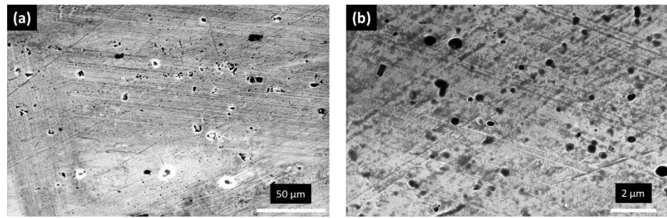
Figure 4. SEM micrograph of as-cast AlSi10Mg alloy at (a) 1800 \times and (b) 30,000 \times magnification.
