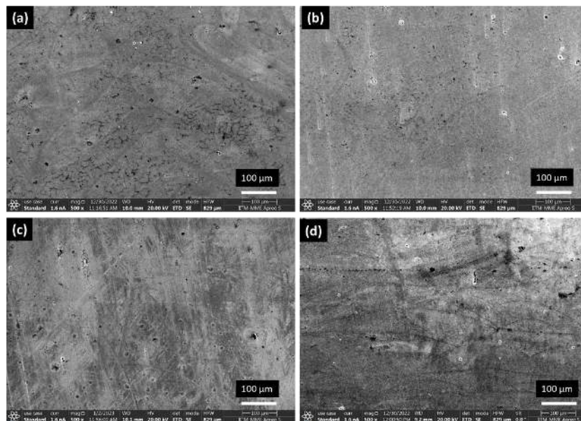
Figure 5. SEM micrographs of (a) horizontally built under Ar; (b) vertically built under Ar; (c) horizontally built under N 2 ; (d) vertically built under N 2 of the SLMed AlSi10Mg alloy at 500 \times magnification.
