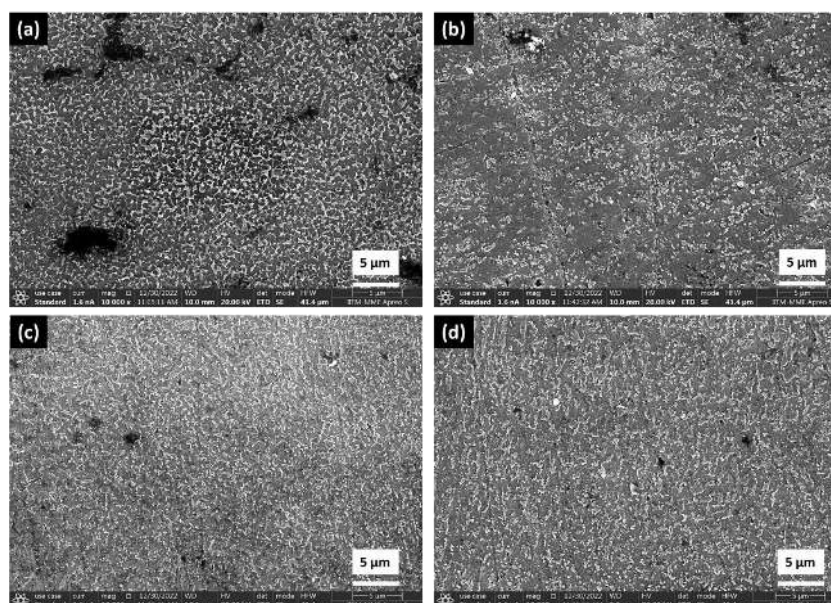
Figure 6. SEM micrographs of (a) horizontally built under Ar; (b) vertically built under Ar; (c) horizontally built under N 2 ; (d) vertically built under N 2 of the SLMed AlSi10Mg alloy at 10,000 \times magnification.
