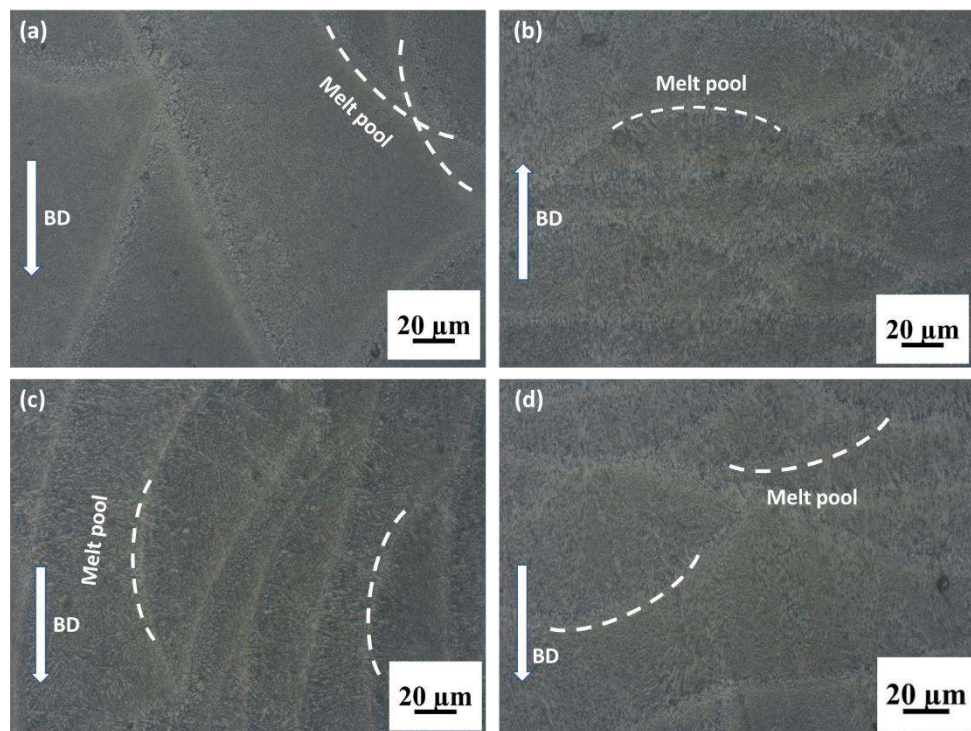
Figure 3. Optical micrographs of (a) horizontally built under Ar; (b) vertically built under Ar; (c) horizontally built under N 2 ; (d) vertically built under N 2 of the SLMed AlSi10Mg alloy. (Note: BD is an abbreviation for built direction).
