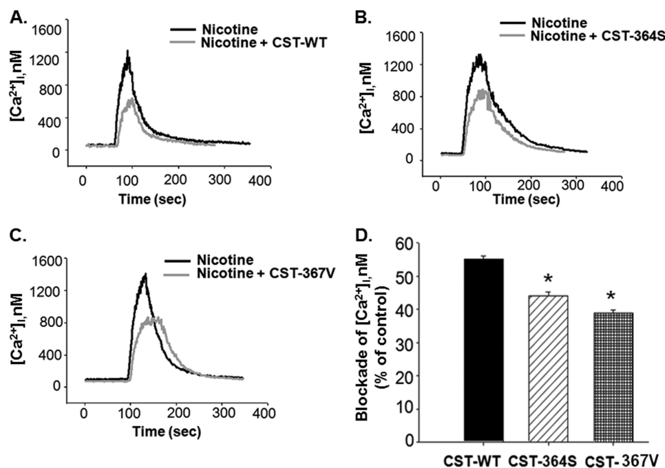
FIGURE 4. CST variants block nicotine-evoked augmentation of cytosolic free calcium concentration. NGF-differentiated PC12 cells loaded with Fura2-AM were stimulated with nicotine (200 μM) in the absence/presence of CST peptides (5.0 μM). The intracellular calcium concentration ( [Ca^{2+}]_i ) values were calculated from the Fura-2 fluorescence. A , B , and C , shown are representative [Ca^{2+}]_i transients in the cases of nicotine (black trace) and CST-WT, CST-Ser-364, and CST-Val-367 (gray traces) respectively. D , the percentage blockade of [Ca^{2+}]_i for each CST peptide was calculated. Data plotted are the mean ± S.E. values from 123 cells for CST-WT, 103 cells for CST-Ser-364, and 90 cells for CST-Val-367. One-way ANOVA followed by Gabriel post hoc tests between the groups suggested significant difference in blocking the nicotine-stimulated calcium rise among the peptides. * indicates p < 0.05 with respect to CST-WT.
