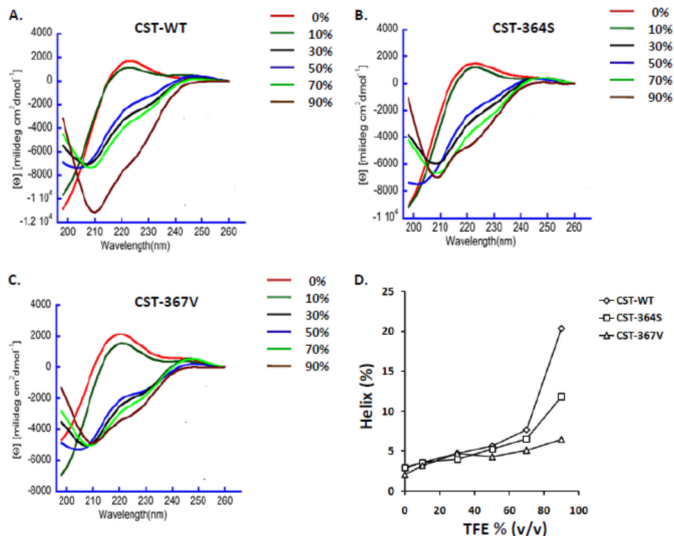
FIGURE 7. CD spectra of the CST variants. CD spectra of the human CST peptides (at 50 \mu M concentration in PBS, pH 7.4) were monitored over a 198–260 nm wavelength in the absence or presence of 10, 30, 50, 70, and 90% TFE. Ascending TFE concentrations induced \alpha -helix formation, as indicated by the two minima at 208 and 222 nm. The representative traces for CST-WT (A), CST-Ser-364 (B), and CST-Val-367 (C) are shown. D, \alpha -helix content for the CST peptides at various TFE concentrations is shown; the data were generated by deconvolution of spectra. The peptides showed altered propensities for formation of \alpha -helix in the following order: CST-WT > CST-Ser-364 > CST-Val-367.
