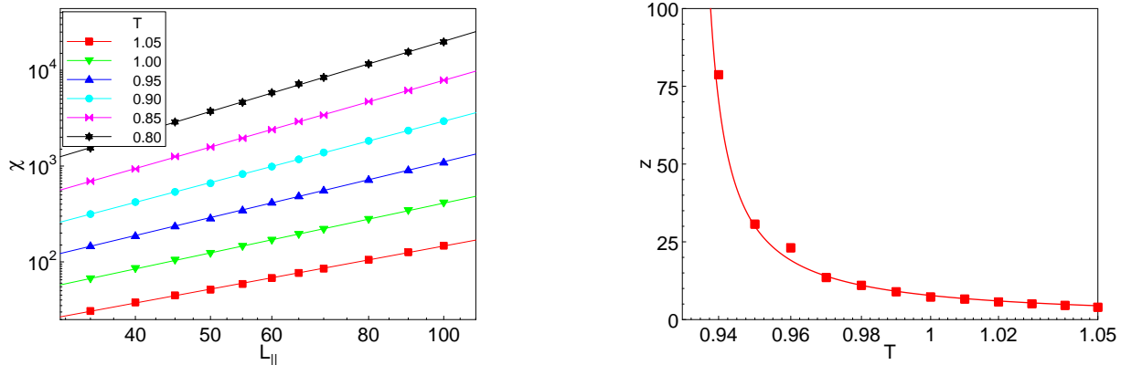
Figure 1. Left: Susceptibility \chi as a function of in-plane system size L_{\parallel} for several temperatures in the Griffiths region. The perpendicular size is L_{\perp} = 800 ; the data are averages over 160 disorder configurations. The solid lines are fits to the power law (3). Right: Resulting Griffiths dynamical exponent z as a function of temperature T in the weakly disordered Griffiths region.
