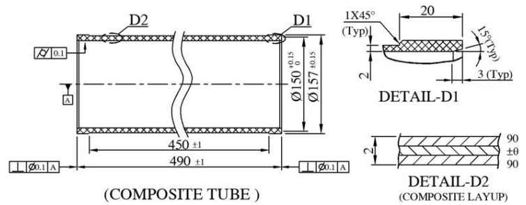
Figure 1. Dimensional details of realised composite tubes.
