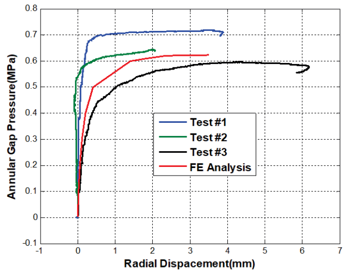
Figure 5. Comparative results of load-deflection of empty tube.
