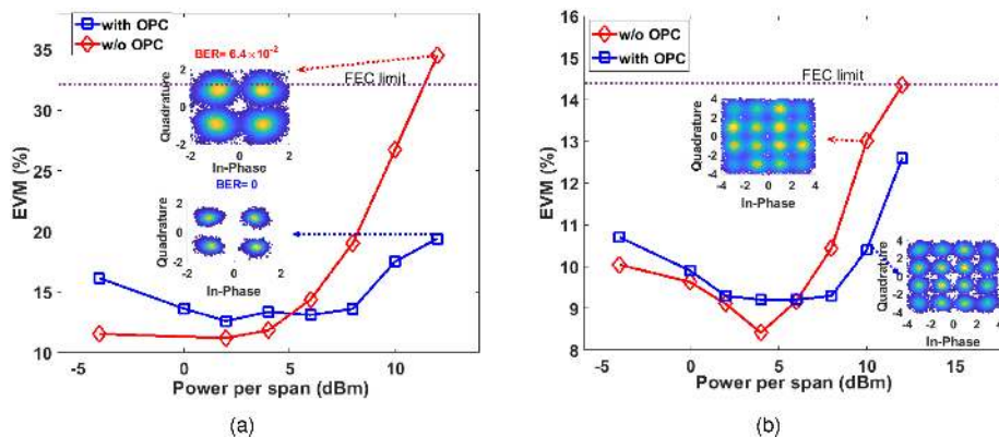
Fig. 3. EVM as a function of input launch power to each 50 km fiber span, in the presence and absence of OPC (a) 40 Gbps QPSK and (b) 80 Gbps 16 QAM.
