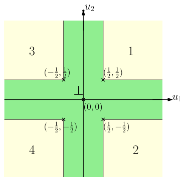
FIG 2. The partition of \mathbb{R}^2 induced by \text{pred}_{\frac{1}{2}}^{\text{BEP}}
