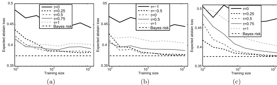
FIG 3. Results on synthetic data: Performance of the CS (left), OVA (middle) and BEP (right) surrogates for various thresholds as a function of training sample size.
