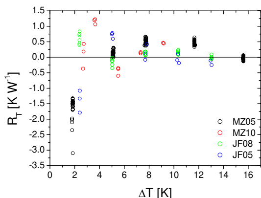
Fig. 6. Thermal resistance derived from four CCNC calibration experiments with ammonium sulfate aerosol at different pressures and flow rates (MZ05, MZ10, JF08, JF05, cf. Table 2) by fitting the CCNC flow model of Lance et al. (2006).
