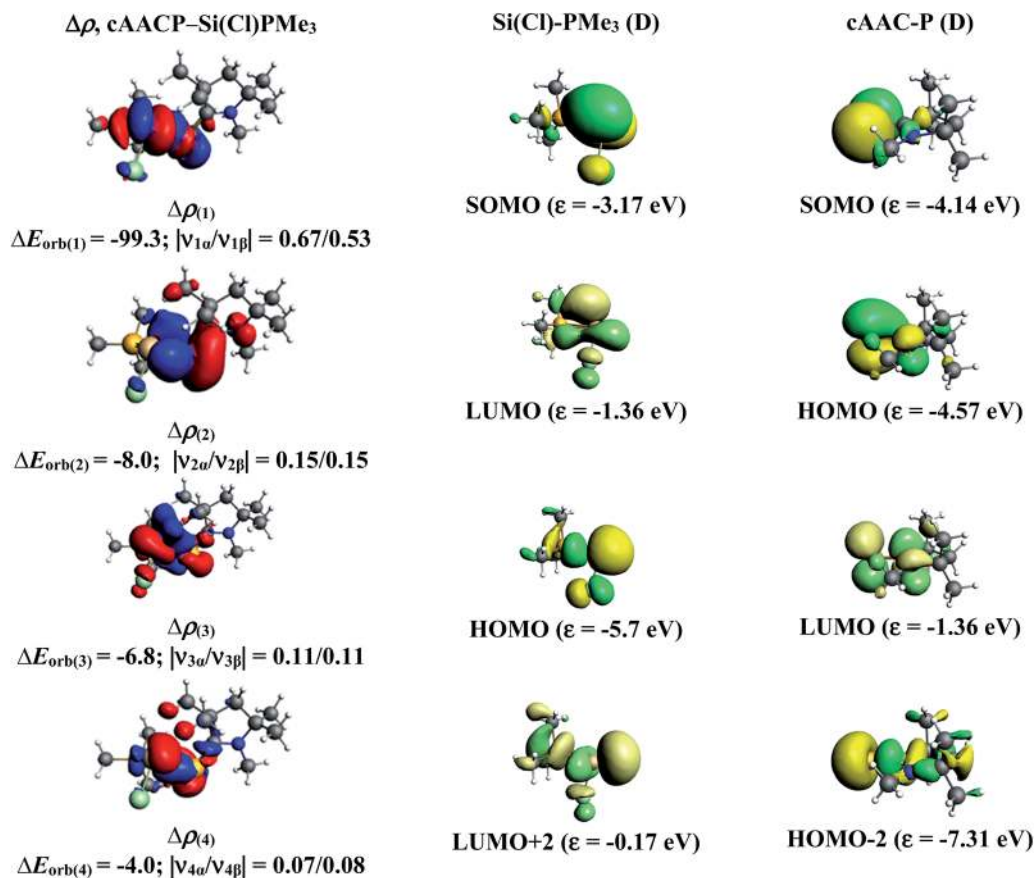
Fig. 8 The shape of the deformation densities, \Delta\rho_{(1)-(4)} that correspond to \Delta E_{orb(1)-(4)} , and the associated MOs of cAAC-P-Si(Cl)-PMe 3 and the fragments orbitals of cAAC-P and (Cl)Si-PMe 3 in the doublet state at the BP86-D3(BJ)/TZ2P level. Isosurface values are 0.003 au. The eigenvalues |v_n| give the size of the charge migration in e. The direction of the charge flow of the deformation densities is red \rightarrow blue.
