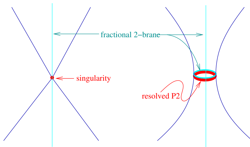
Figure 1: A schematic description of the fractional two-branes both before and after the singularity is resolved.
