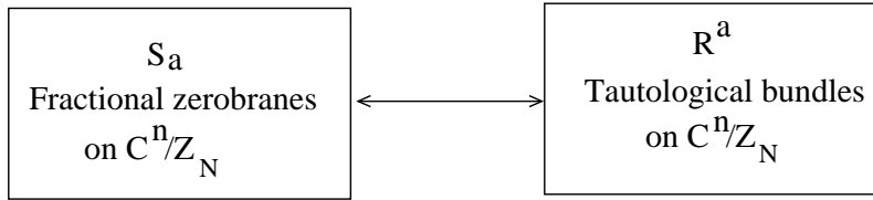
Figure 2: The McKay correspondence for \mathbb{C}^n/\mathbb{Z}_N .
