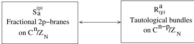
Figure 3: The proposed quantum McKay correspondence for \mathbb{C}^n/\mathbb{Z}_N .
