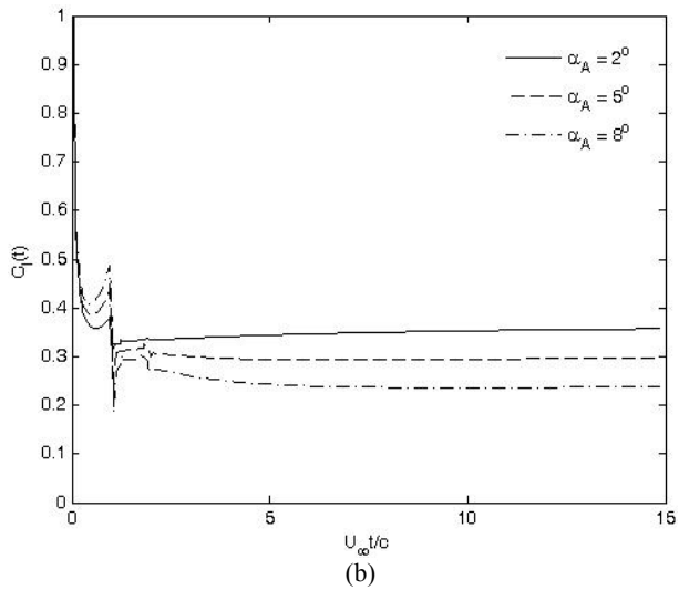
Fig. 17: C_l(t) for (X_0, Y_0) = (2c, 0) , V_A = V_B = 27\text{m/s} , \alpha_B = 4^\circ (a) airfoil A and (b) airfoil B
