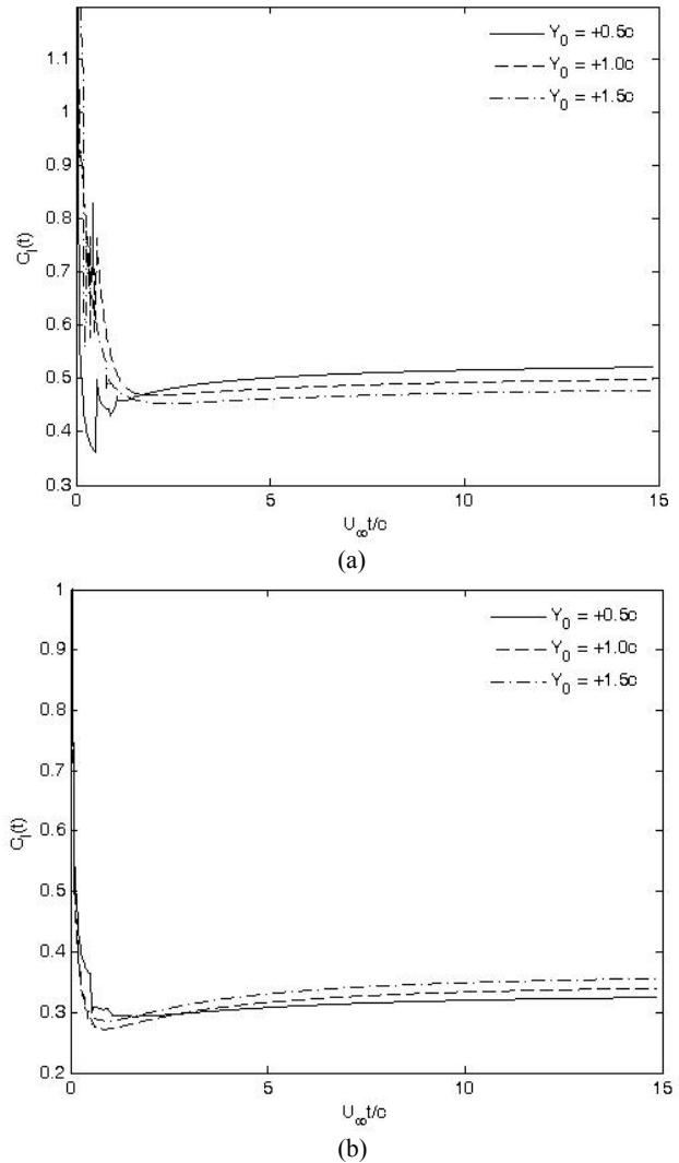
Fig. 13: C_l(t) for X_0 = 2c , \alpha_A = \alpha_B = 4^\circ , V_A = V_B = 27\text{m/s} (a) airfoil A and (b) airfoil B
