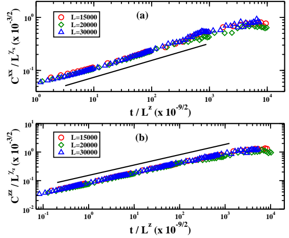
FIG. 3: (color online). Log-log plots of C^{xx} (top) and C^{zz} (bottom) as functions of t/L^z , showing data collapse on to single curves after scaling.
