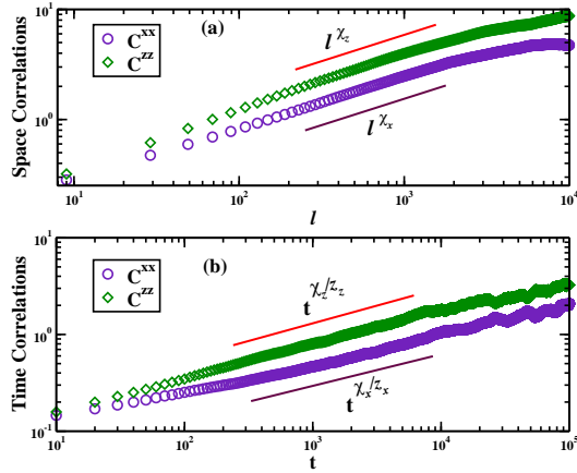
FIG. 2: (color online). Log-log plot of equal-time correlators C^{xx}(l, t = 0) and C^{zz}(l, t = 0) versus spatial separation l (top) and (b) log-log plots of equal space-point time-dependent correlators C^{xx}(l = 0, t) and C^{zz}(l = 0, t) versus t . Slopes yield exponents \chi_x, \chi_z and \chi_x/z_x, \chi_z/z_z , respectively (see text).
