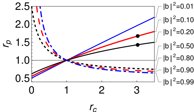
FIG. 3. (Colour online) The variation of r_p = P_2/P_3 is shown with the ratio of overlaps, r_c = c_2/c_1 corresponding to different values of |b|^2 . Different curves correspond to different values of |b|^2 , that are specified on the right side of the plot. Two black points on the curves for |b|^2 = 0.1, 0.2 correspond to experimental conditions of the datasets numbered 7 and 8 of Table I.
