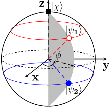
FIG. 4. (Colour online) Bloch sphere representation of |\psi_1\rangle , |\psi_2\rangle , and |\chi\rangle , marked with unfilled red circle, filled blue circle, and filled black square respectively.
