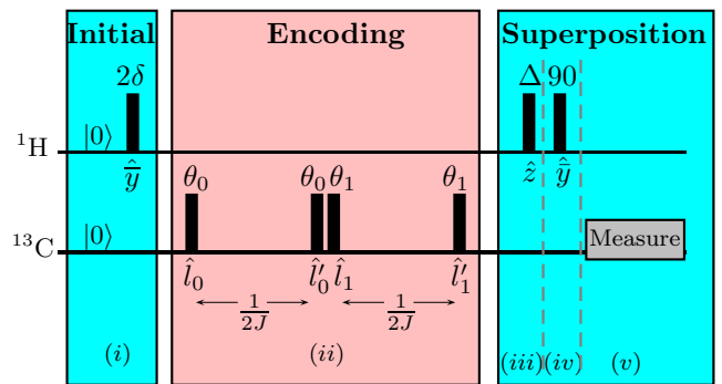
FIG. 1. (Colour online) NMR pulse sequence to obtain a superposition of two single-qubit states starting with the pseudo-pure state |00\rangle . The two channels show the operations on ancilla ( ^1\text{H} ) and system qubits ( ^{13}\text{C} ) respectively. Pulse sequence is divided into three parts, shown as separate blocks of different colors. Also, various steps are numbered from (i)-(v). The radio-frequency pulses are shown as rectangles, with respective angles of rotations mentioned at the top and the axes of rotations specified at the bottom. The arbitrary rotation axes are \hat{l}_0 = \cos(\frac{3\pi}{2} + \phi_0)\hat{x} + \sin(\frac{3\pi}{2} + \phi_0)\hat{y} , \hat{l}'_0 = \cos(\phi_0)\hat{x} + \sin(\phi_0)\hat{y} , \hat{l}_1 = \cos(\pi + \phi_1)\hat{x} + \sin(\pi + \phi_1)\hat{y} , and \hat{l}'_1 = \cos(\frac{\pi}{2} + \phi_1)\hat{x} + \sin(\frac{\pi}{2} + \phi_1)\hat{y} . At the end of the sequence, a single-qubit measurement is performed on the system qubit.
