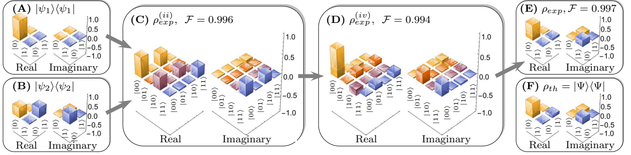
FIG. 2. (Colour online) (A) and (B) show the theoretical input states from dataset 3 of Table I, part (C) contains the two-qubit state after encoding ( \rho_{exp}^{(ii)} ), (D) represents the state obtained at the end of step ( iv ) of the pulse sequence ( \rho_{exp}^{(iv)} ), parts (E) and (F) show the final experimentally obtained ( \rho_{exp} ) corresponding to step ( v ) and theoretically expected ( \rho_{th} ) single-qubit superposed states respectively.
