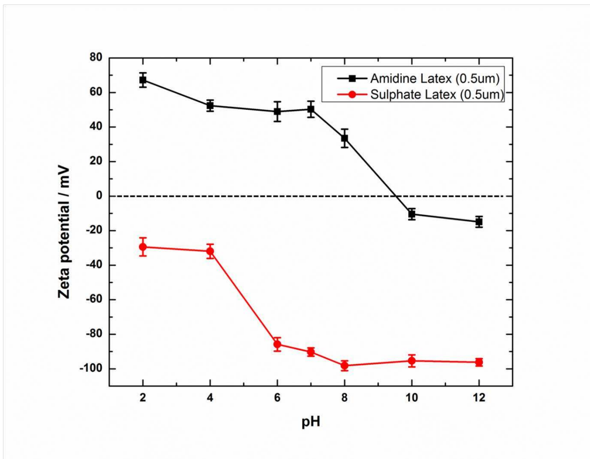
Figure S8. Zeta-potential of pure amidine (0.5 \mu\text{m} ) and sulphate (0.5 \mu\text{m} ) polystyrene particles at different pH. Sulphate-coated particles remained stable over the whole pH range. Amidine-coated particles were stable over the pH range of 2 to 8 but aggregated at pH 10 and 12.
