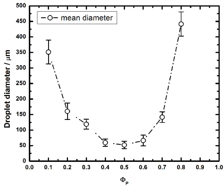
Figure S6. Variation of average droplet diameter of o/w emulsions ( \phi_o = 0.05 ) formed in vials shown in Figures 7 and 8 of main text versus \phi_p . Error bars represent standard deviation.
