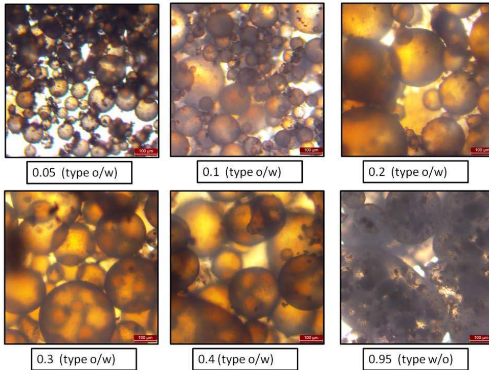
Figure S5. Representative optical microscopy images of emulsion droplets formed in vials shown in Figure 4 of main text. The numbers refer to fraction of oil phase \phi_o . An increase in droplet size was observed towards phase inversion. The average drop diameter ranged from 105 \mu\text{m} at \phi_o = 0.05 to 350 \mu\text{m} at \phi_o = 0.4 . Scale bar = 100 \mu\text{m} .
