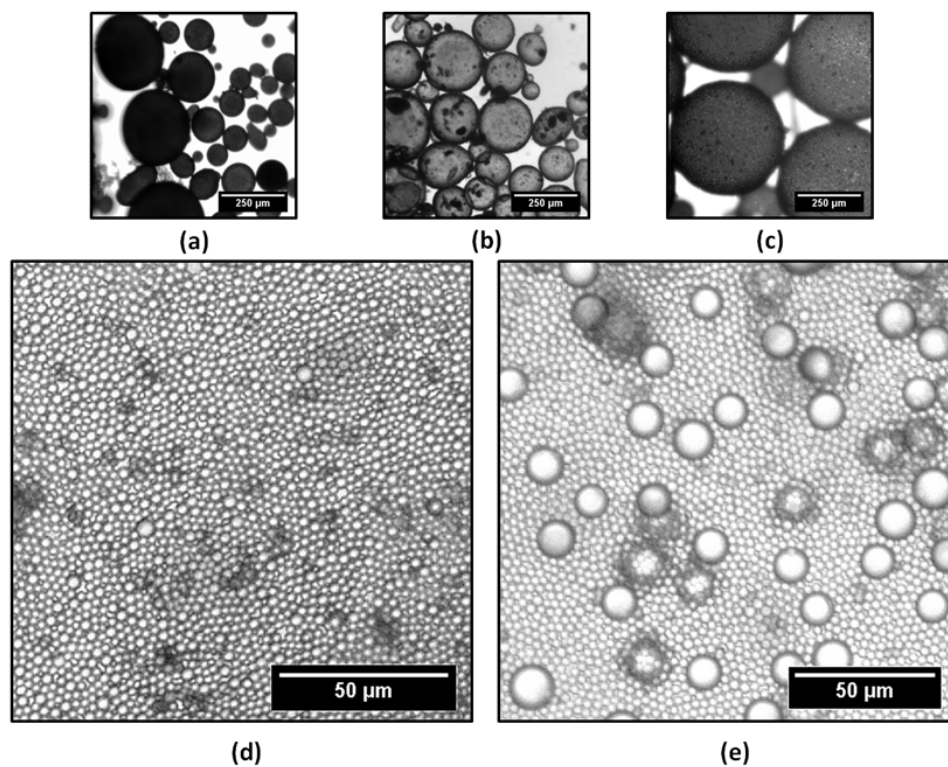
Figure S7. Emulsification of aqueous dispersions of OCP of polystyrene latex of different sizes. All emulsions are w/o ( \phi_o = 0.9 ). (a) Mixture of 2.2 \mu\text{m} (+)/3.0 \mu\text{m} (-) particles, (b) mixture of 0.5 \mu\text{m} (+)/0.5 \mu\text{m} (-) particles, (c) mixture of 2.2 \mu\text{m} (+)/9.0 \mu\text{m} (-) particles. Close up of the surfaces of a water drop in oil are shown in (d) corresponding to system in (a), and in (e) corresponding to system in (c) respectively. Ratio of positive:negative particles used are (a) 1:1, (b) 1:2 and (c) 17:1 respectively.
