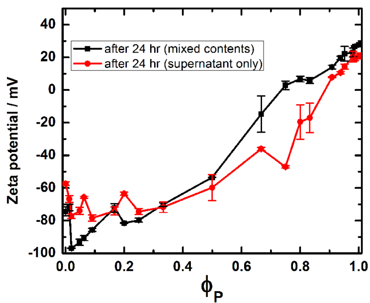
Figure S2. Zeta potential of mixtures of OCP shown in Figure S1 measured after 24 hr, both of the supernatant and the homogeneous dispersion.
