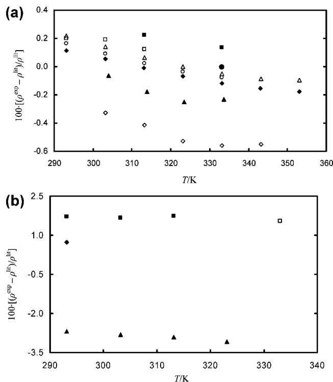
Figure 2. Relative deviations between the experimental density data of this work and those reported in the literature as a function of temperature. (a) [C 2 mim][NTf 2 ] at 0.10 MPa: ▲, Fredakle et al.; 19 □, Noda et al.; 44 ◆, Krummen et al.; 49 ●, Lopes et al.; 50 ○, Hong et al.; 51 △, Jacquemin et al. 52 [C 8 mim][NTf 2 ] at 0.10 MPa: ◇, Kato and Gmehling; 53 ■, Aki et al. 54 (b) [C 2 mim][BF 4 ] at 0.10 MPa: ■, Noda et al.; 44 □, Van Valkenburg et al.; 48 ◆, Zhao et al.; 55 ▲, Zhang et al. 56
