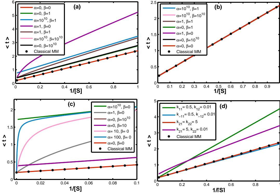
FIG. 3: Single-enzyme Lineweaver-Burk plots for \langle t \rangle v versus 1/[S] for the parallel pathway MM mechanism (in non-dimensional units) for (a) different rates of enzymatic interconversion characterized by the rate constants \alpha and \beta for k_{21} \neq k_{22} , (b) same as (a) but in the absence of asymmetry in the rate constants for the catalytic steps k_{21} = k_{22} , (c) different rates of conformational fluctuations arising solely from enzyme or enzyme-substrate interconversion characterized by the rate constants \alpha or \beta respectively and (d) asymmetry in the rate constants for substrate binding, substrate release or catalytic steps. Common parameter values in (a)-(d) are k_{11} = k_{-11} = k_{12}^{(d)} = k_{-12}^{(d)} = 0.5 , k_{21} = 5 , k_{22}^{(b),(d)} = 0.1 and \alpha = \beta = 1^{(a),(b),(c)} . The parameter values which were varied in subfigures (a)-(d) are indicated as superscripts and the corresponding values are indicated as subfigure legends. For the chosen parameter values in (a), the green, black and pink curves almost merge onto each other. Filled circles correspond to the mean turnover time [Eq. (9)] for the (single-pathway) MM mechanism [Eq. (1)] with k_1 = k_{-1} = 0.5 , k_2 = 5 .
