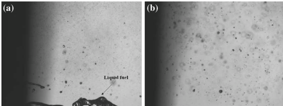
Figure 13. State of the charge exiting the carburettor at (a) Idling, (b) Full throttle under unsteady pressure variation. Each image spans a region of 5\text{ mm} \times 4\text{ mm} at the exit of the carburettor.
