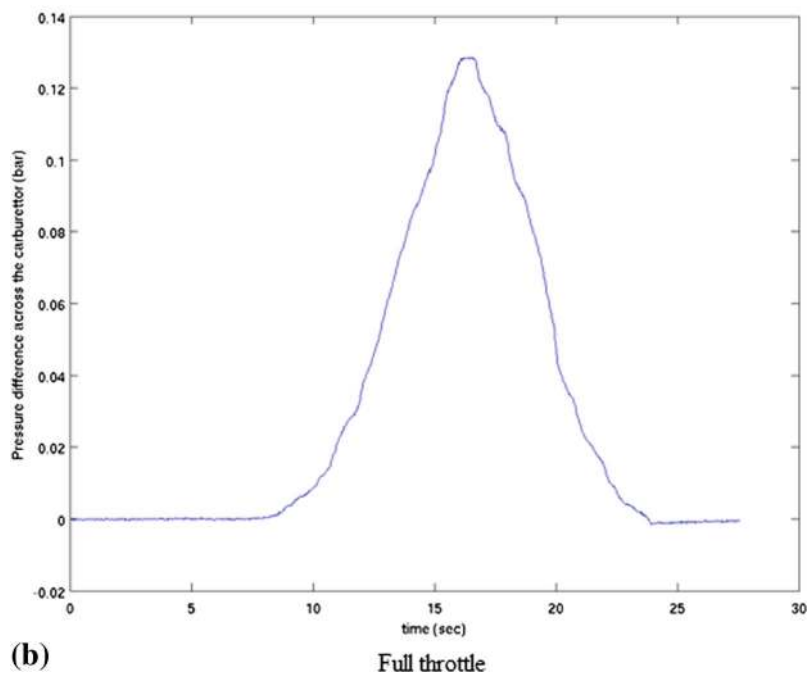
Figure 12. Pressure difference measured across the carburettor during (a) Idling throttle and (b) Full throttle position.
