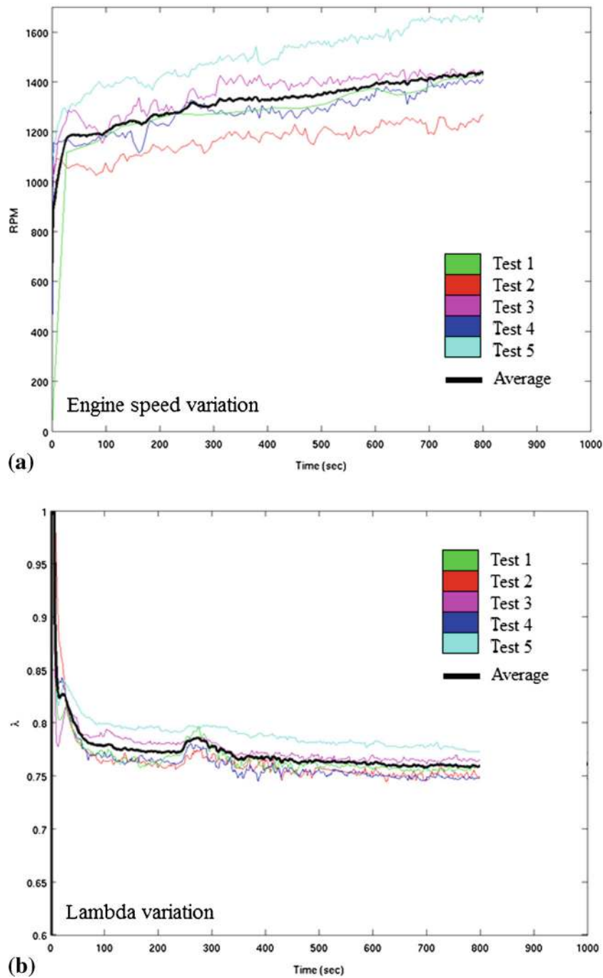
Figure 17. Lambda ( \lambda ) variations at 35°C preheated case for different days with the engine speed variation with the corresponding colours.
