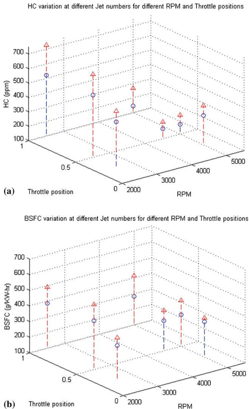
Figure 18. Comparison of (a) HC emissions and (b) Brake specific fuel consumption for Jet I (circle) and Jet II (triangle) nozzle diameter cases for various load and speed combinations. The vertical lines show the position on the x-y plane.
