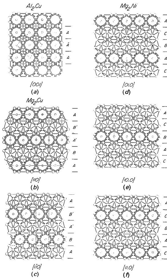
Fig. 1. The structures of (a) tetragonal Al 2 Cu along [001]; orthorhombic Mg 2 Cu along (b) [110] and (c) [1 \bar{1} 0]; and hexagonal Mg 2 Ni along (d) [01.0], (e) [10.0] and (f) [11.0].
