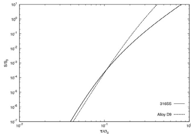
Fig. 2. Variation of grain boundary sliding rate with resolved shear stress following Horton's formula. The testing temperatures are 873K for 316SS and 973K for alloy D9.
