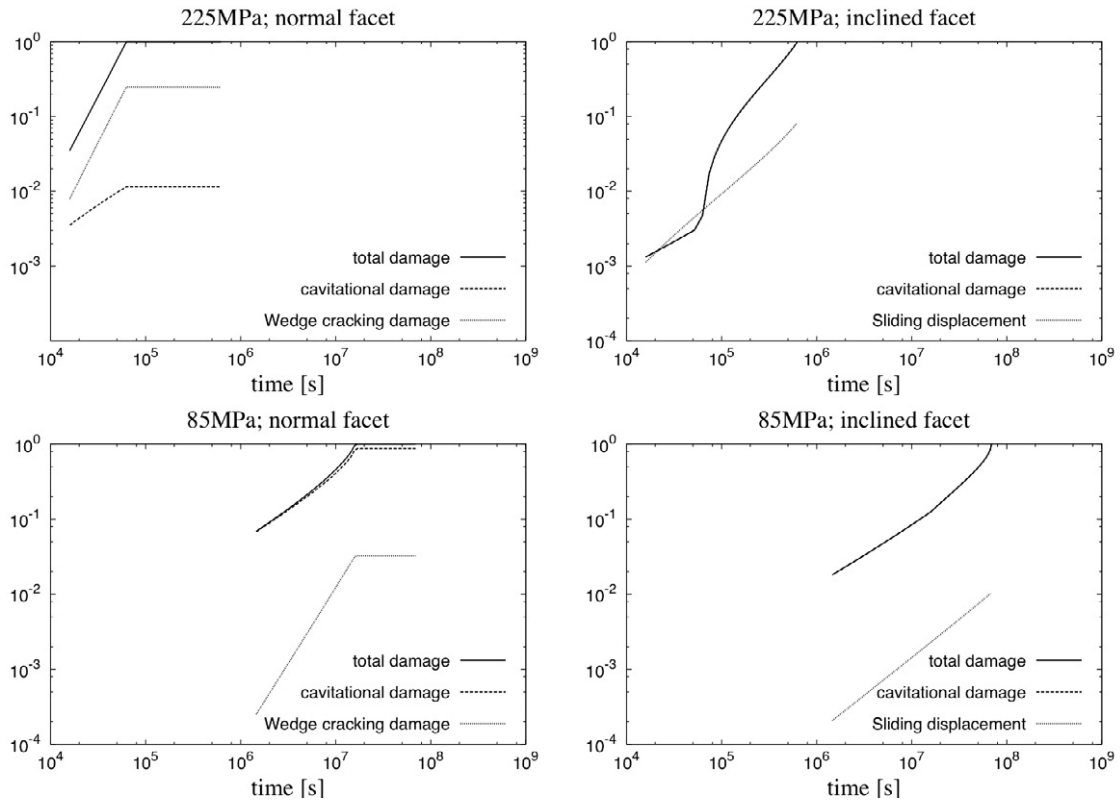
Fig.3. Evolution of damage in alloy D9 at two stress levels (225 MPa and 85 MPa) in the normal facets (left column) and in the inclined facets (right column).
