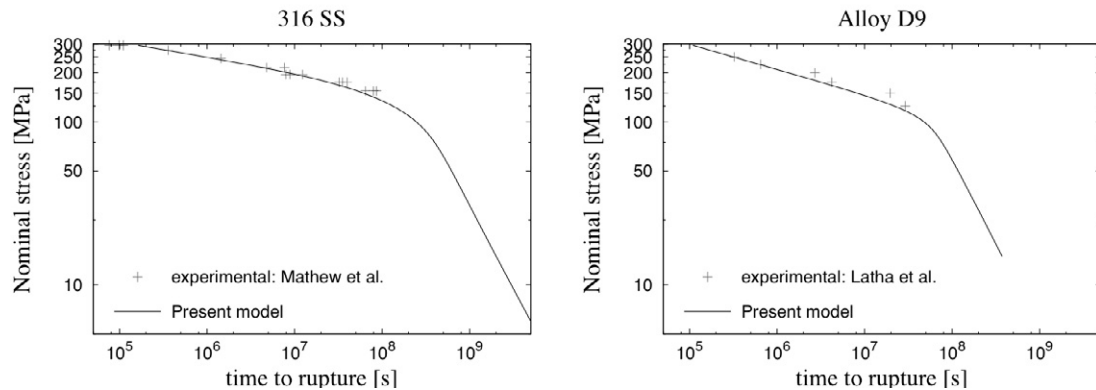
Fig. 1. Comparison of the experimental and predicted time to rupture for 316SS and alloy D9.
